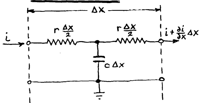
(b) ELECTRICAL
