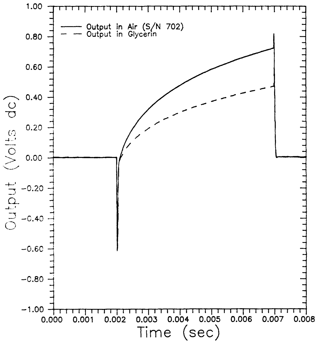
Figure B.1 \text{Sqrt}(\rho C_p k) Calibration Output for Gauge No. 1
