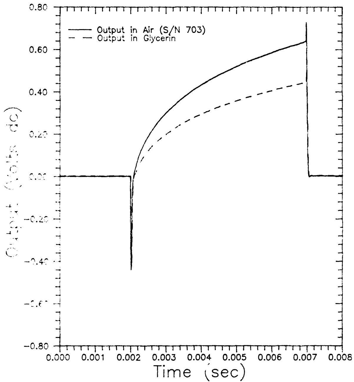
Figure B.11 \text{Sqrt}(\rho C_p k) Calibration Output for Gauge No. 6
