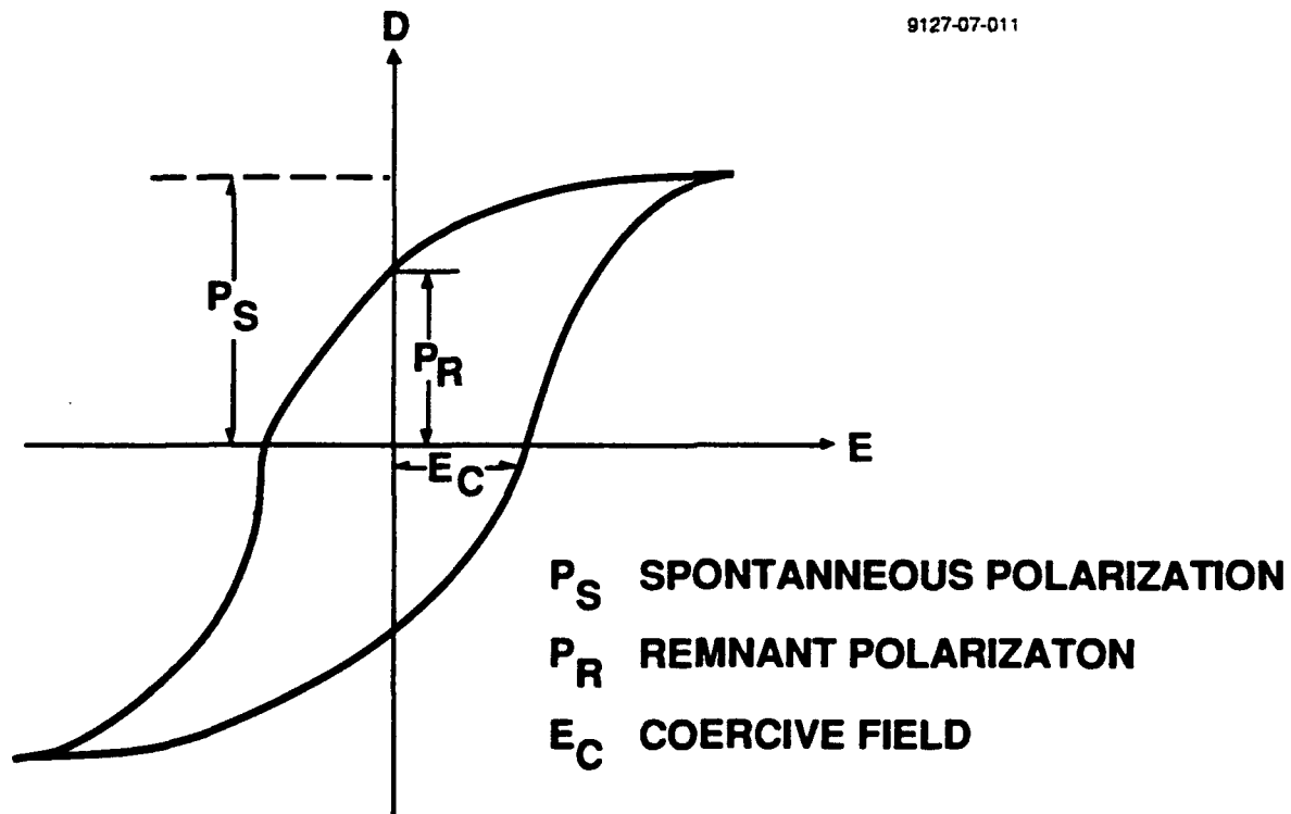
Fig. 54. Ideal hysteresis loop.
