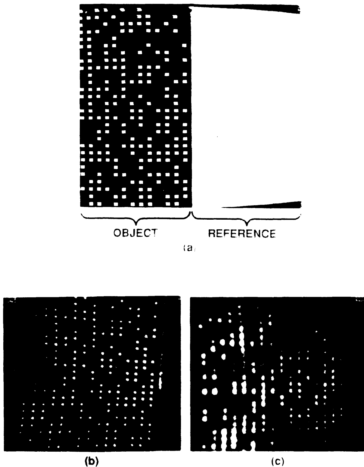
Fig. 26. Experimental demonstration of fanout and global connectivity using fanned reference beam. (a) Object and reference used for recording. (b) Hologram of object using 100% of original reference. (c) Hologram reconstructed using 0.9% of original reference showing fanout of 1:110 and global connectivity. Demonstration of larger fanout was limited by CCD sensitivity.
