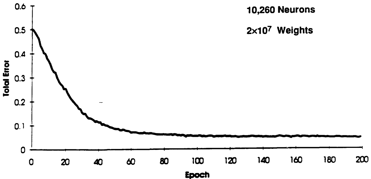
Fig. 43. Multi-output-neuron single-layer optical Perceptron learning of 4 exemplars. The network consisted of 6840 input neurons, 3420 output neurons, and 2 \times 10^7 connection weights.
