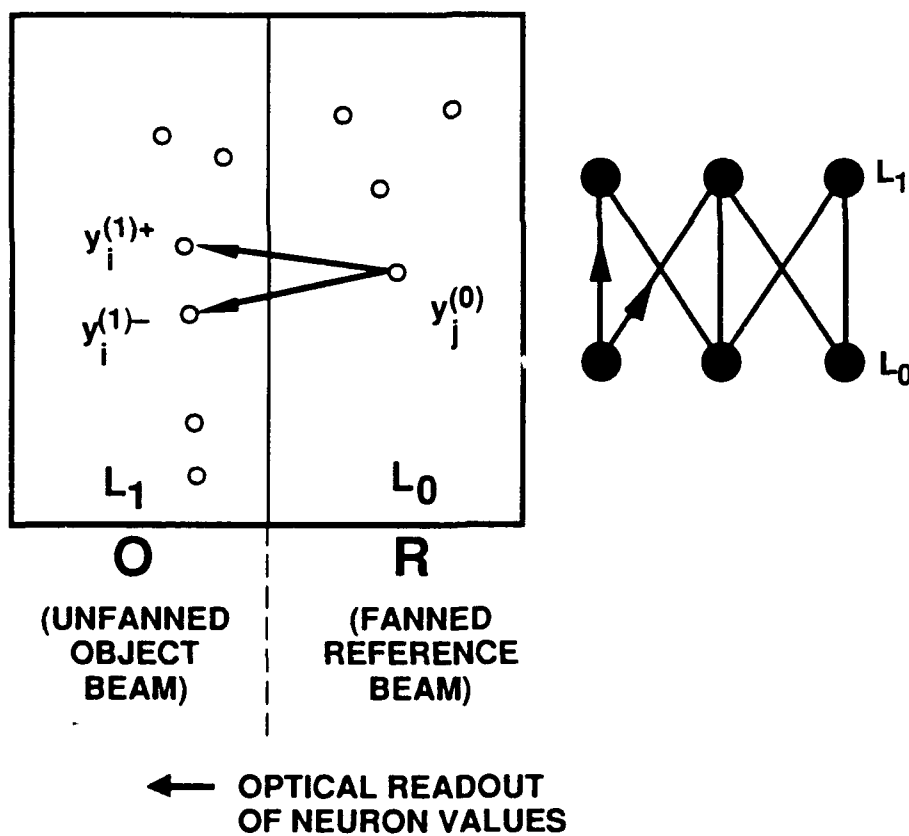
Fig. 39. Optical input plane for single layer Perceptron.
