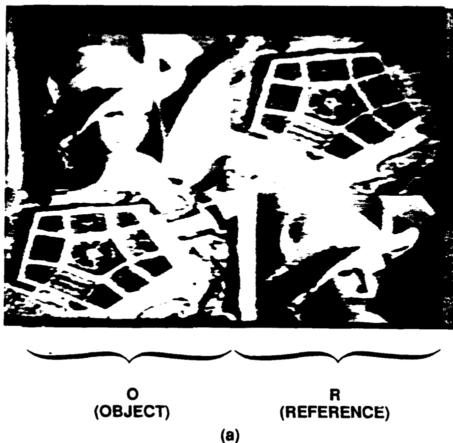
Fig. 24. Experimental demonstration of recorded image quality using fanned reference beam and 2-D non-sampled reference. (a) Object and reference used for recording.
