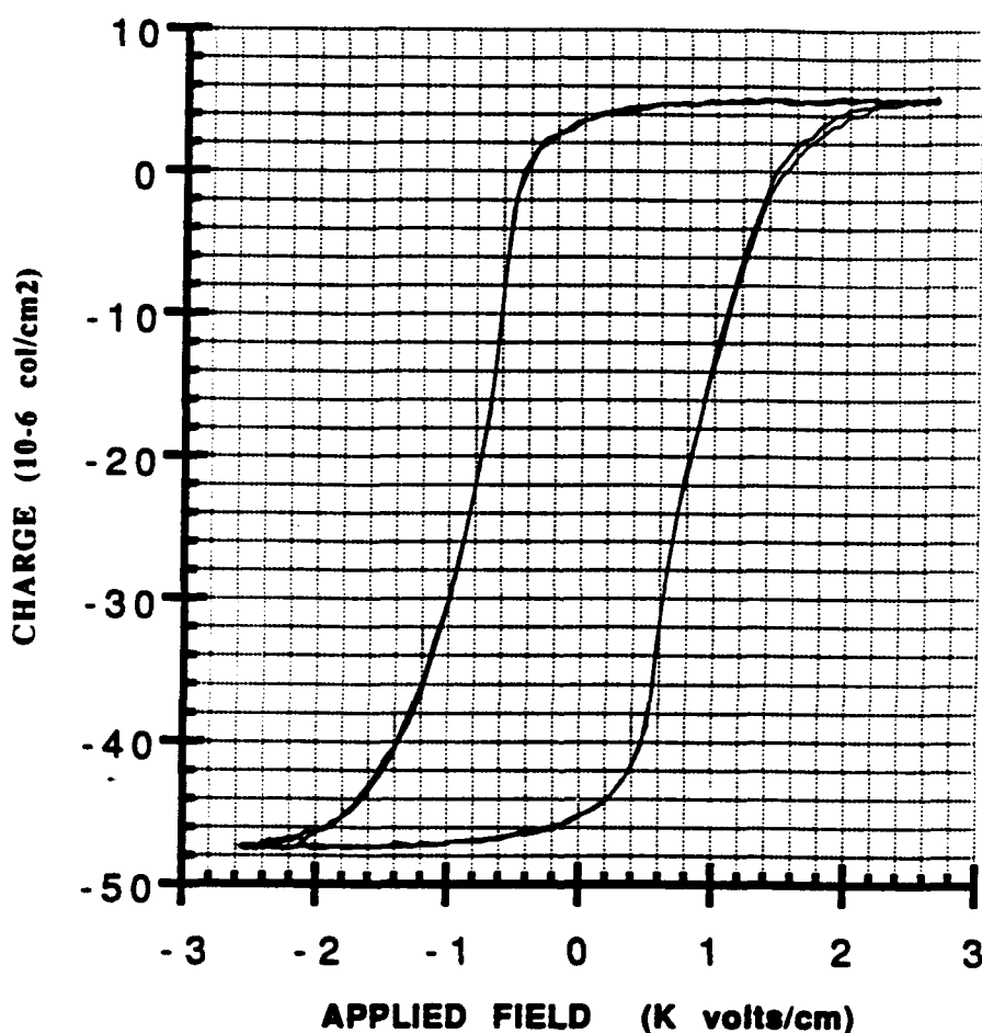
Fig. 55. Measured hysteresis loop of \text{BaTiO}_3 crystal.
