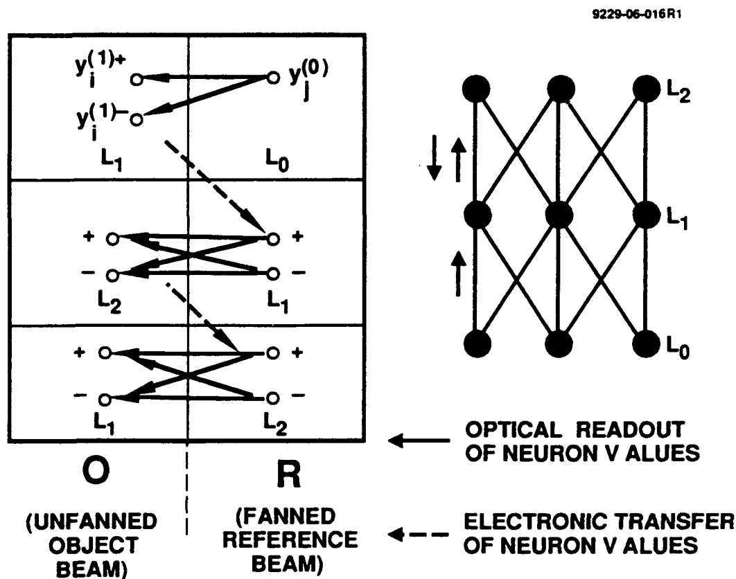
Fig. 46. Optical input plane for optical backpropagation with a single hidden layer.
