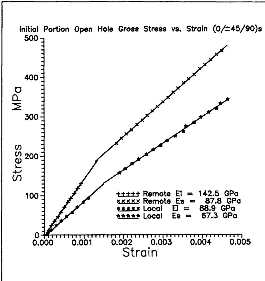
Figure 34 Initial Portion of Stress-Strain Curves [0/\pm 45/90]_s
