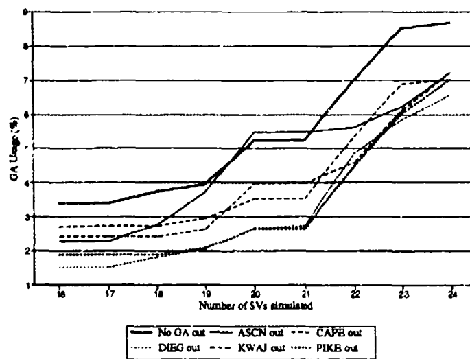
Figure 4.19. Percentage of Time Three GAs in Simultaneous Use.
