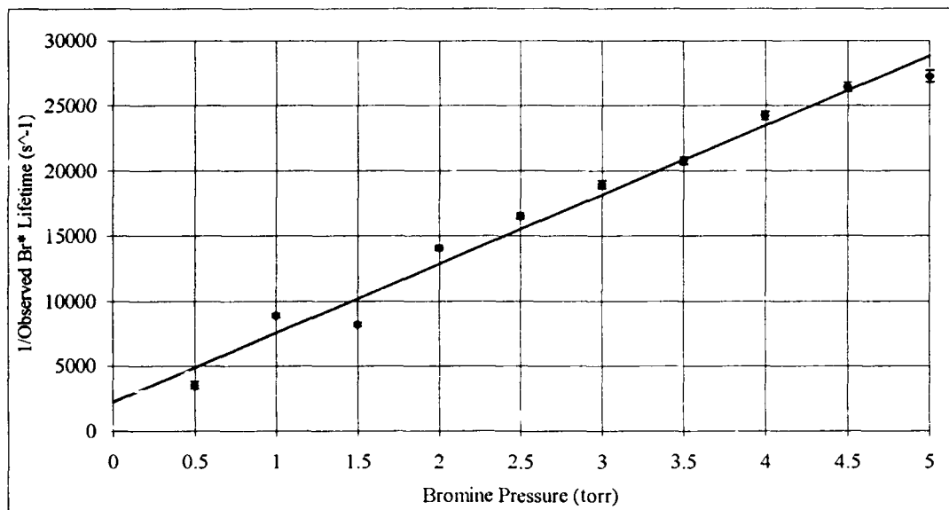
Figure 5.2 Stern - Volmer Fluorescence Lifetime Rate Analysis
