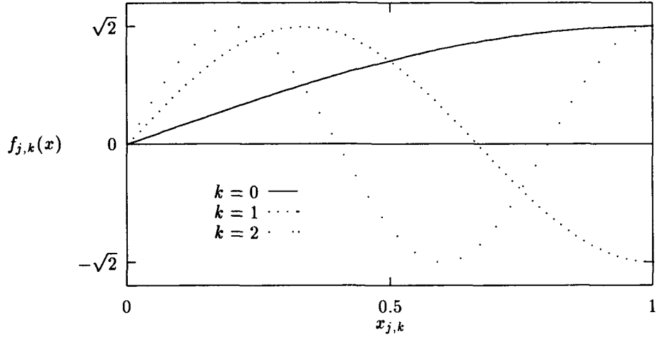
Figure 2.2. Sinusoidal Basis Functions: k = 0, 1, 2 over Normalized Interval
