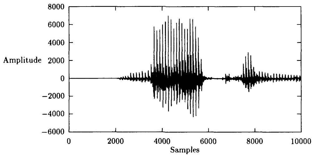
Figure 4.23. Polynomial Fit Output Waveform with 85.0% Compression
