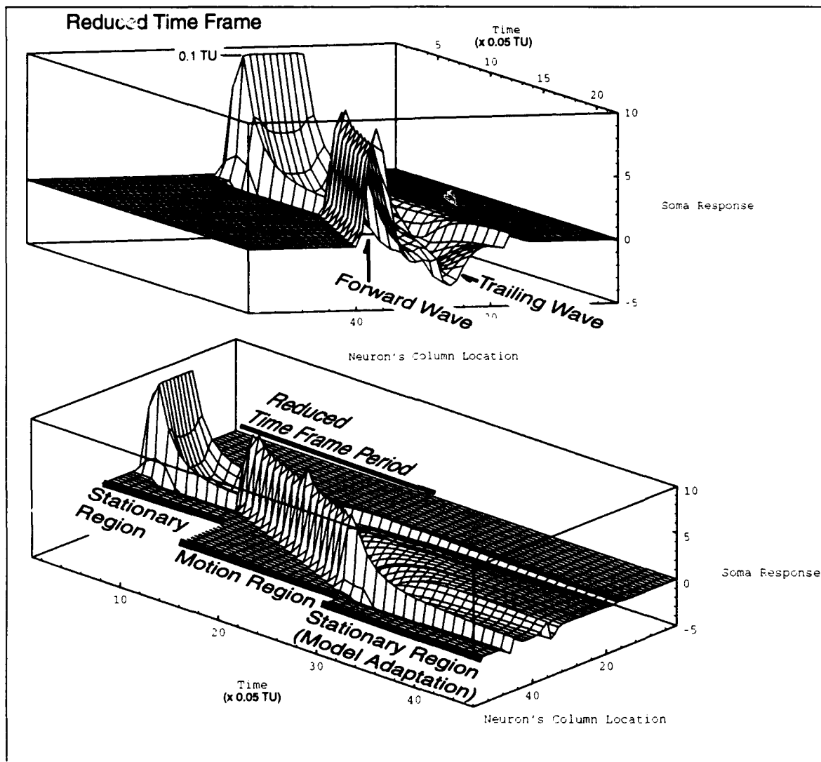
Figure 3.17. This figure shows how the adaptive asynchronous model responds to the rectangular input (RECT). The lower graphic is the full model output and the upper graphic is a short period extracted to show the form of the wave at some time during the motion period. These figures show the model adapting shortly after the introduction of the stationary RECT. When the RECT moves, the model response increases momentarily and begins to adapt once again. In this figure, the jagged edges of the motion wave are caused by our discrete model. The mesa and the forward and trailing waves are illustrated here as well. In the final TUs, the model adapts to the stationary RECT.
