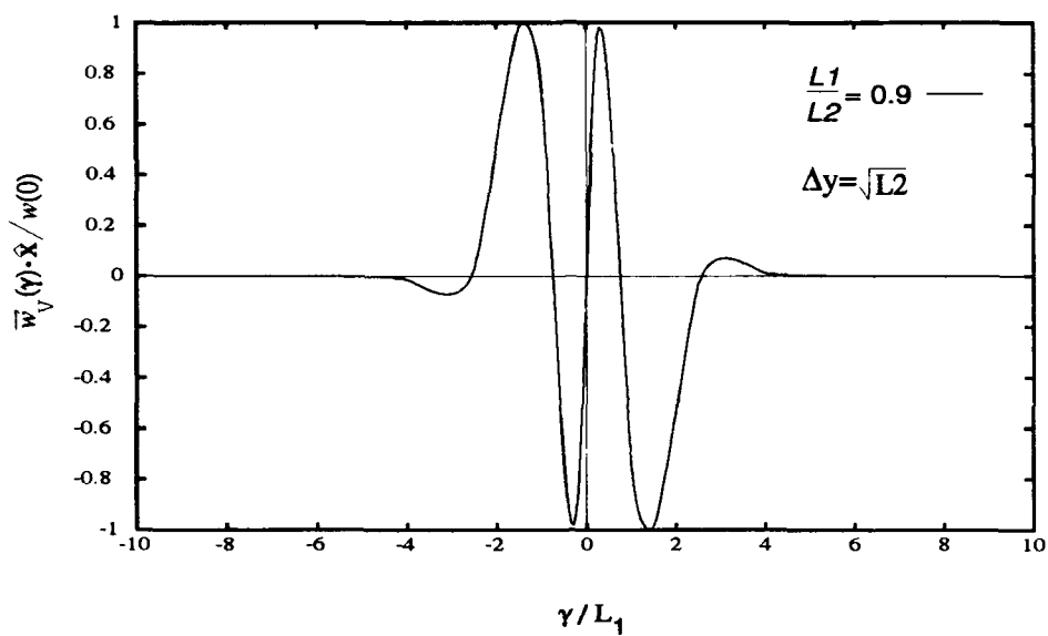
Figure 3.7. x -Directed Component of the Wind Path Weighting Function \vec{w}_V
