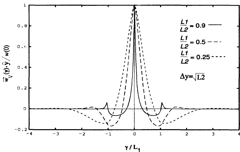
Figure 3.8. y -Directed Component of the Wind Path Weighting Function \vec{w}_V
