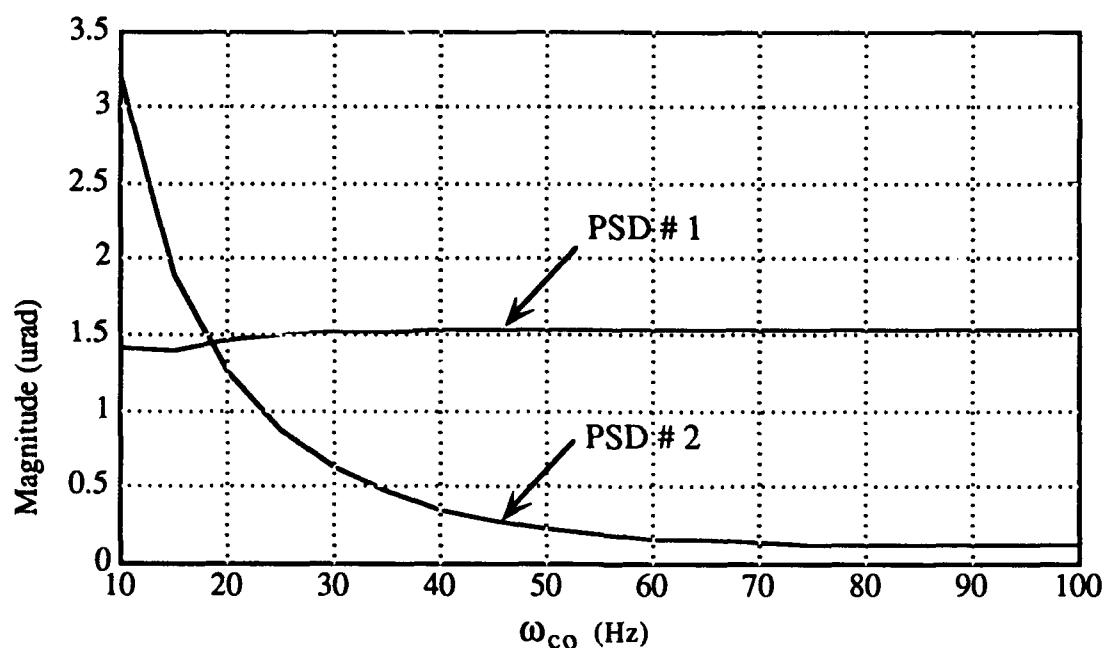
Figure 5.4-11. Shift portion of the residual RMS imaging error, e_1 , versus compensator parameter, \omega_{co} , for measured case-to-rotor coupling.
