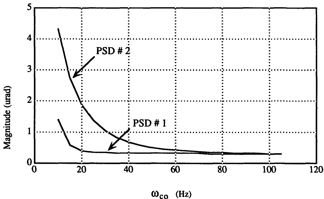
Figure 5.4-1. Residual RMS imaging error versus compensator parameter, \omega_{co} , for ideal case-to-rotor isolation.
