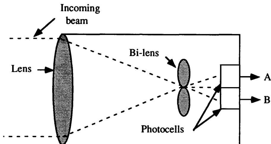
Figure 2.3-1. Simplified diagram of a single axis DYNAC.
