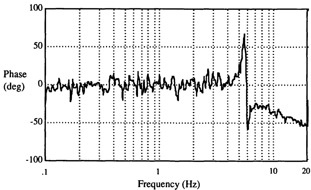
Figure 6.2-5. Measured isolation transfer function phase.
