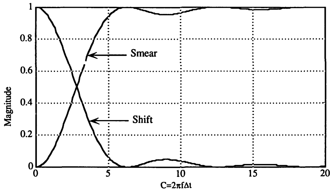
Figure 5.4-8. Weighting function plots.
