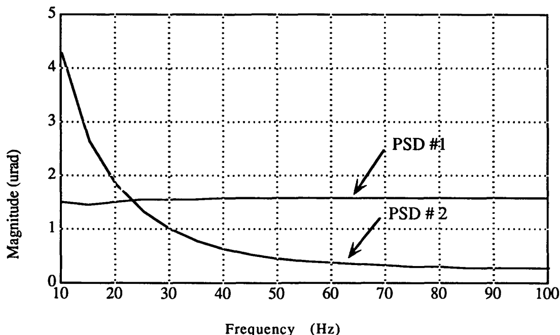
Figure 5.4-7. Residual RMS imaging error, e_1 , versus compensator parameter, \omega_{co} , for measured case-to-rotor coupling.
