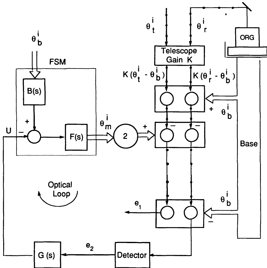
Figure 3.5-1. Image stabilization block diagram.
