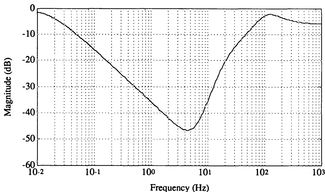
Figure 5.4-2. Magnitude plot of transfer function e_1/\theta_b^1 including analytic case-to-rotor coupling.
