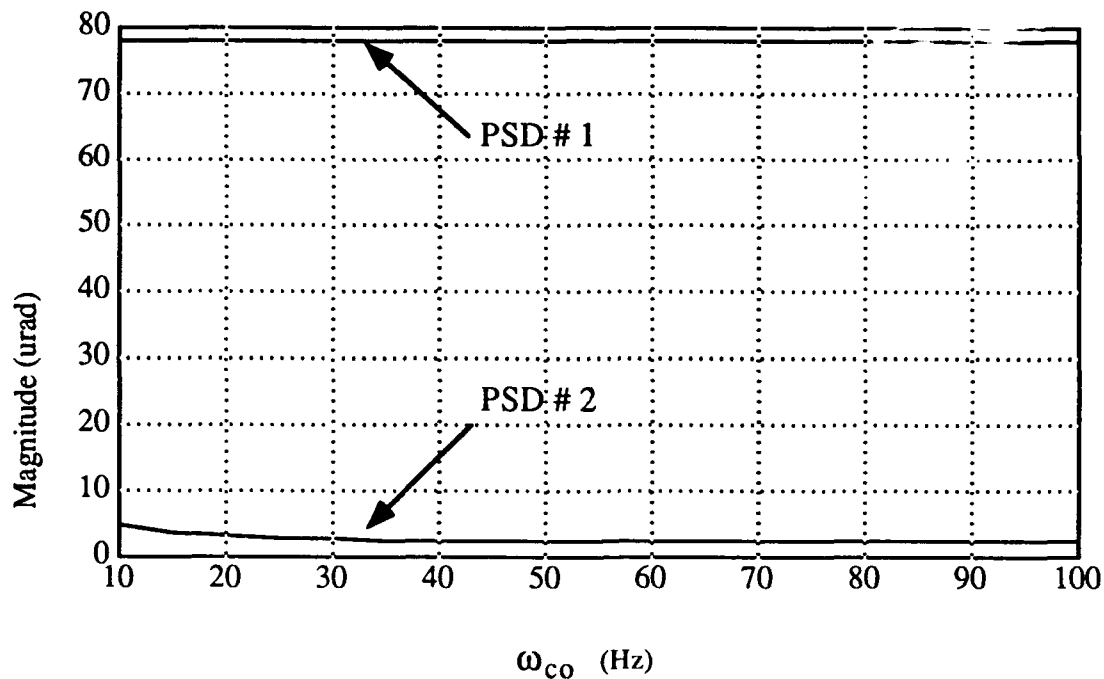
Figure 5.4-3. Residual RMS imaging error, e_1 , versus compensator parameter, \omega_{co} , with analytical case-to-rotor coupling.
