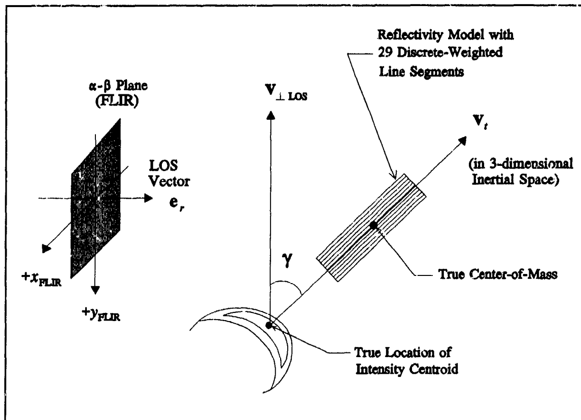
Figure 3.4 3-d Hardbody Reflectivity Model Relative to FLIR Image Plane
