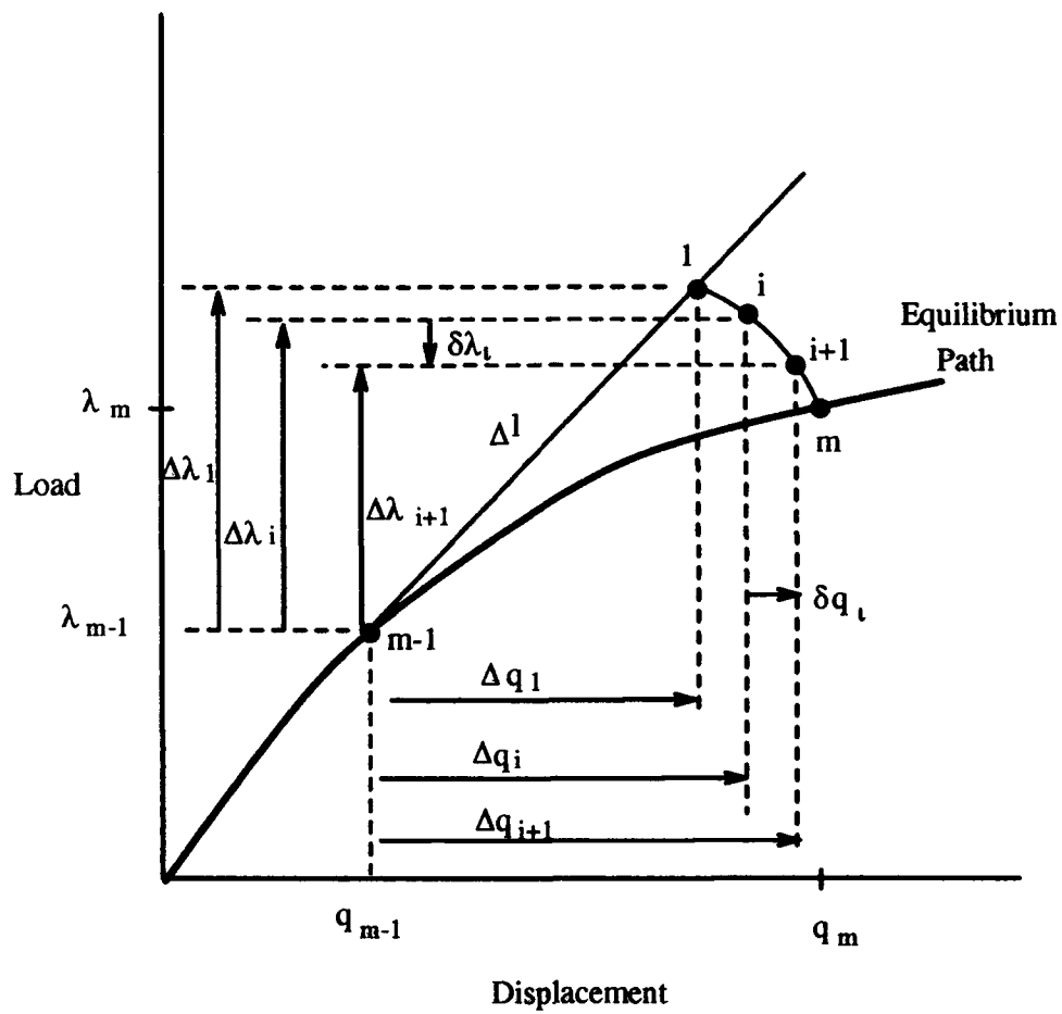
Figure 2.7. Riks Technique
