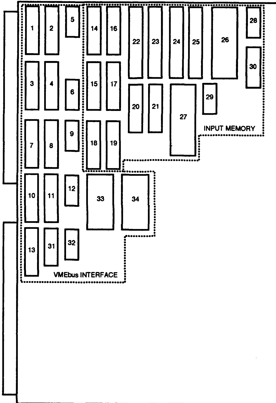
Figure 52. Layout of VME Board # 1
