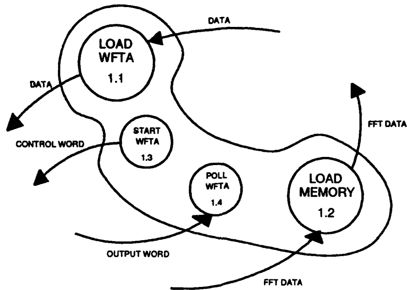
Figure 19. Level 1 DFD for Host Driver Program
