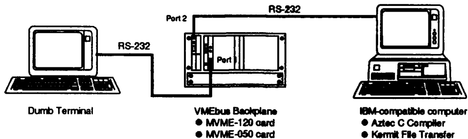
Figure 56. Hardware Setup
