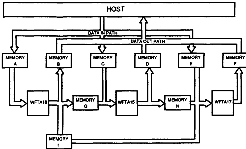
Figure 4. Reconfigurable WFTA Architecture
