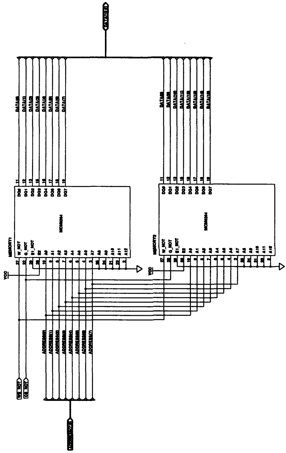
Figure 28. MEM_MCM6264 Block Schematic-Input and Output Memory
