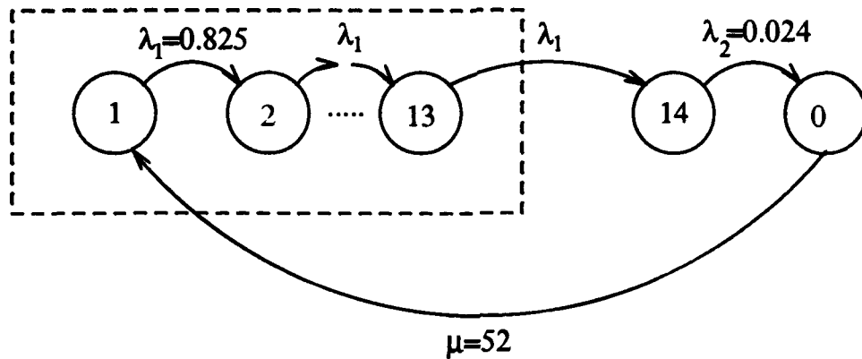
Figure D.5. State Transition Diagram for Stage 2/3 Liner Debond
