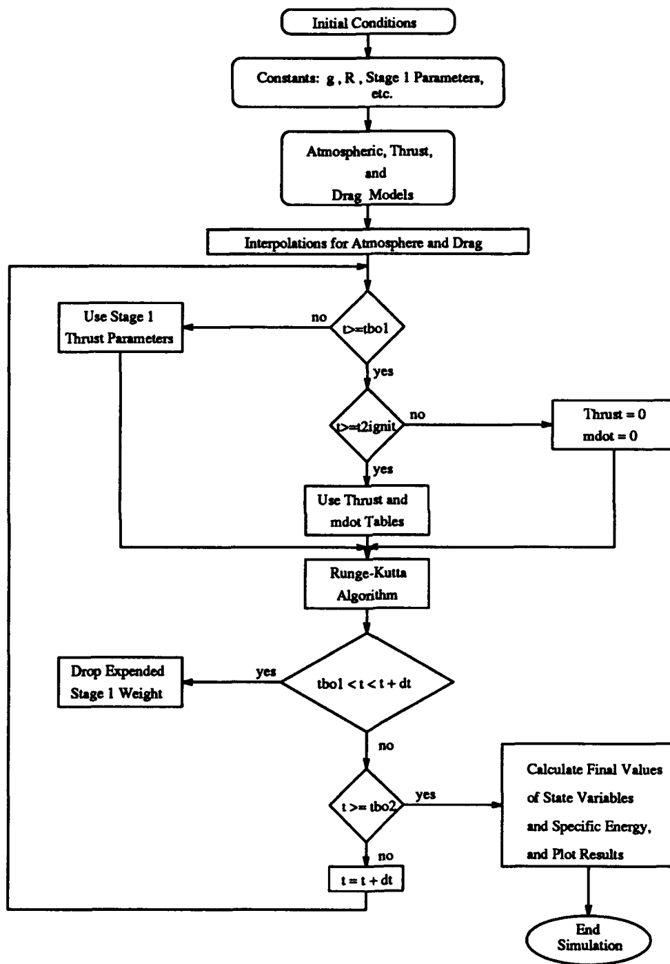
Figure 3.3. TPS Flowchart
