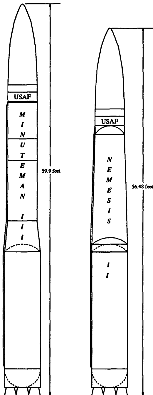
Figure 6.2. Opt 2 - ISC Conical NEMESIS Design
