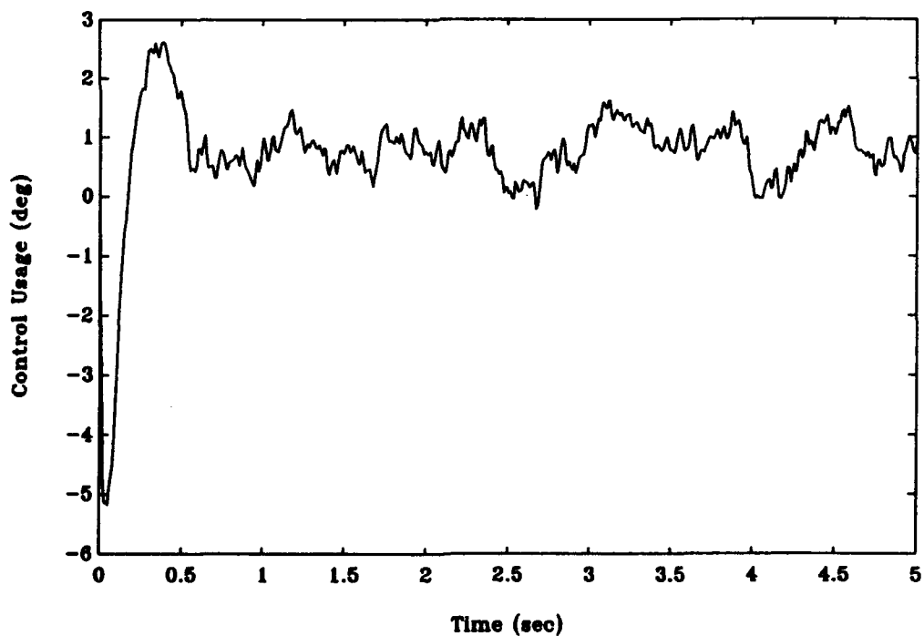
Figure 5-23. Control Usage (u) from N_2 Step, LO, 10% Suboptimal
