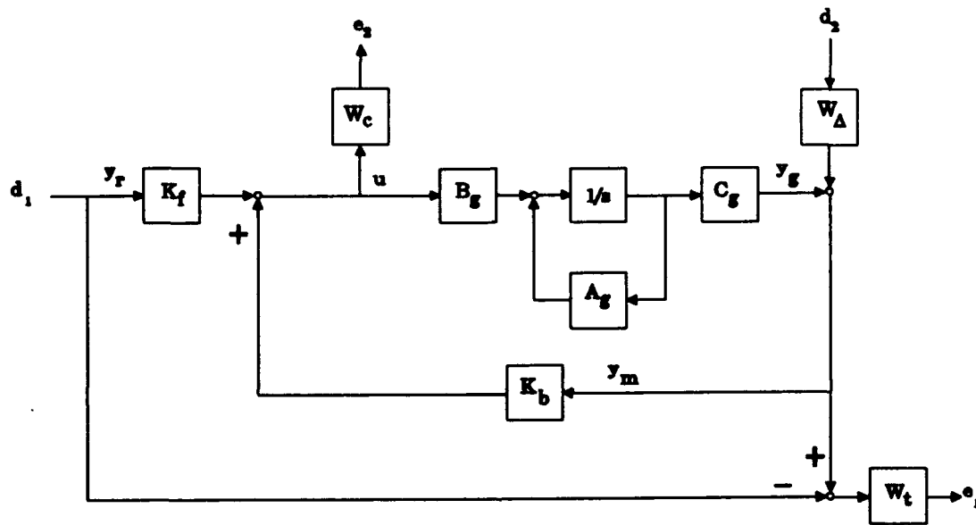
Figure 5-1. H_\infty Robust Tracker Design Diagram
