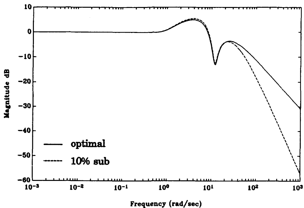
Figure 5-17. Complimentary Sensitivity Magnitude, LO
