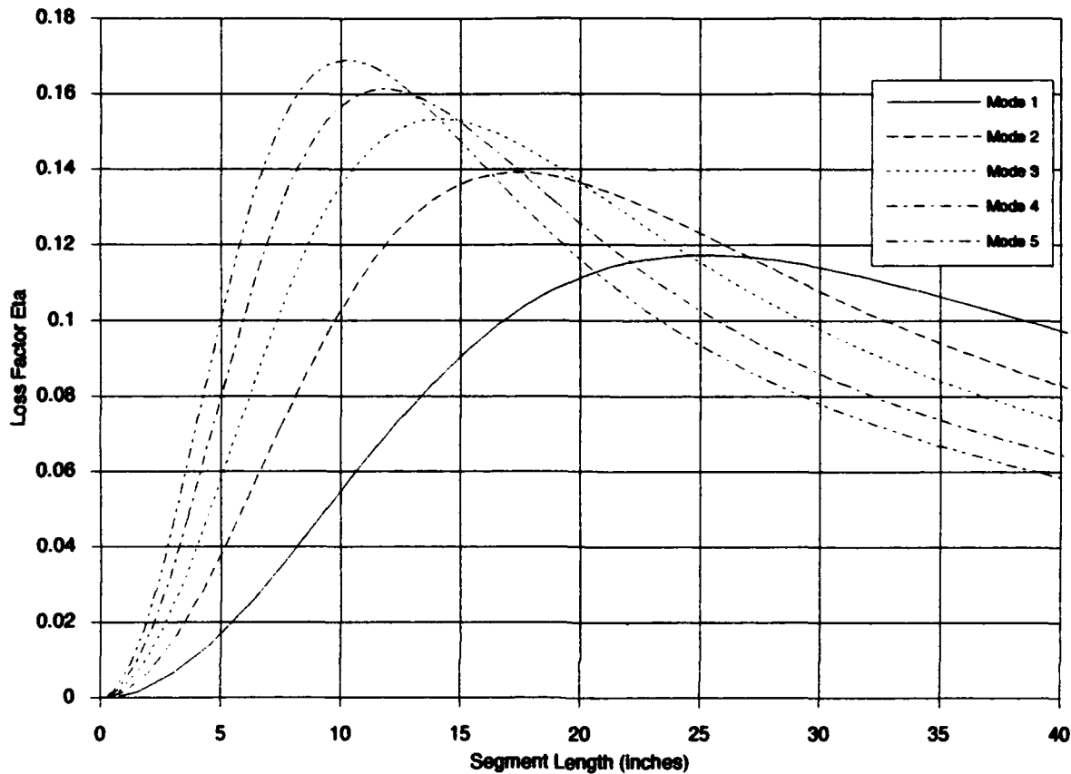
Figure 4.2 Theoretical Loss Factor vs. Segment Length for 032005 ISD 112
