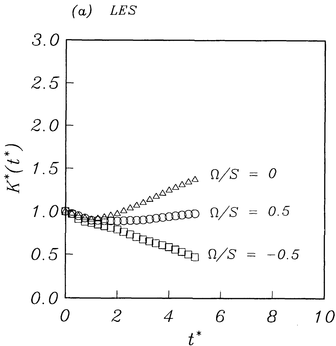
Figure 3. Time evolution of the turbulent kinetic energy in rotating homogeneous shear flow: (a) large-eddy simulations of Bardina et al. (1983), (b) new explicit algebraic stress model, and (c) standard K - \varepsilon model.
