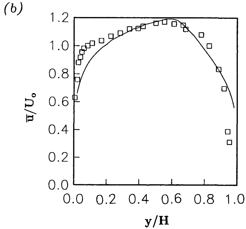
Figure 5. Comparison of the model predictions (-) for the mean velocity profile with the experimental data ( \square ) of Johnston et al. (1972) for rotating channel flow ( Re = 11,500 , Ro = 0.21 ): (a) SSG second-order closure (taken from Speziale et al. 1992) and (b) new explicit algebraic stress model.
