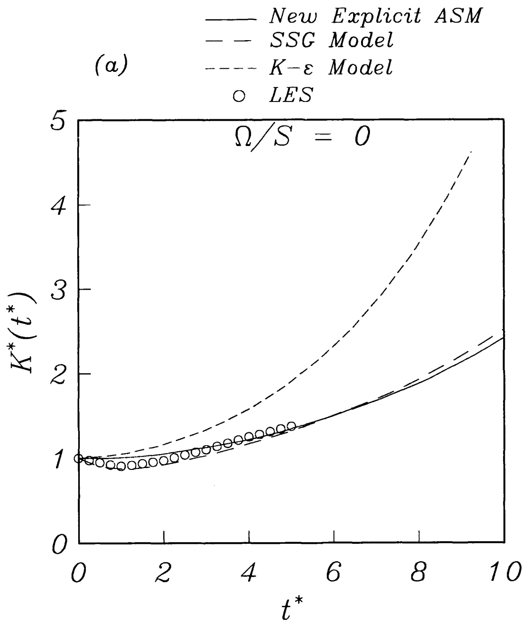
Figure 2. Time evolution of the turbulent kinetic energy in rotating homogeneous shear flow: Comparison of the model predictions with the large-eddy simulations of Bardina et al. (1983). (a) \Omega/S = 0 , (b) \Omega/S = 0.5 and (c) \Omega/S = -0.5 .
