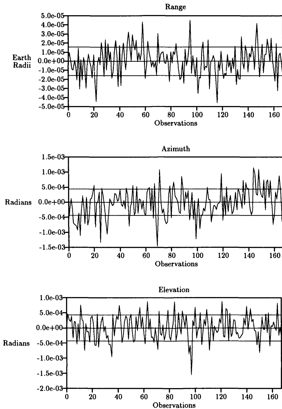
Figure 14. Residual Values versus 1-\sigma After Convergence — Cosmos
