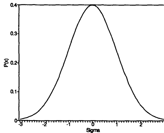
Figure 1. Gaussian Distribution
