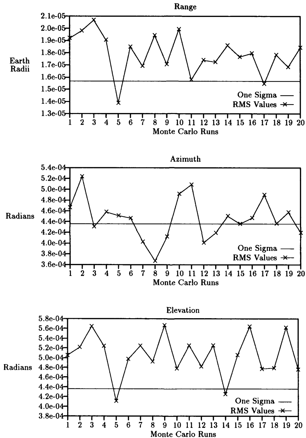
Figure 23. Converged RMS Values versus 1\text{-}\sigma — Explorer
