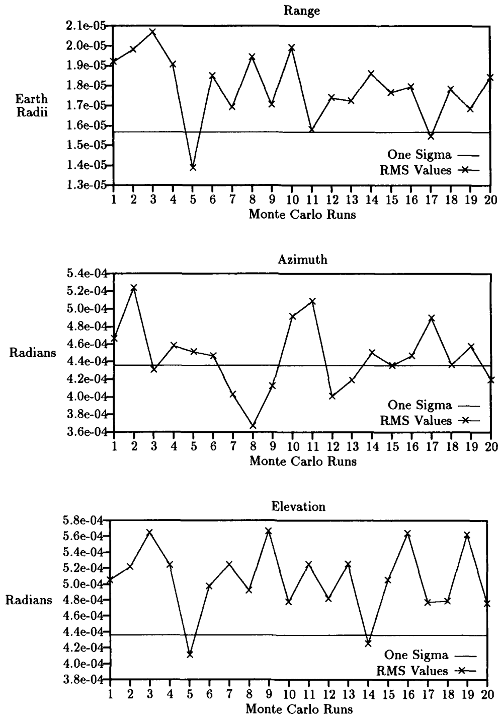
Figure 25. Converged RMS Values versus 1\text{-}\sigma — Full Integrator
