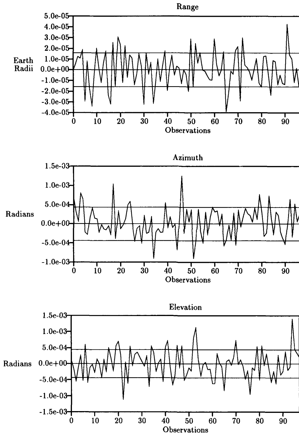
Figure 10. Residual Values versus 1\text{-}\sigma After Convergence — GPS
