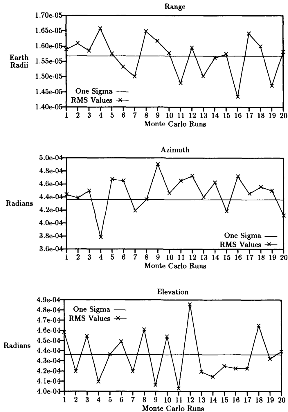
Figure 16. Converged RMS Values versus 1\text{-}\sigma — Cosmos
