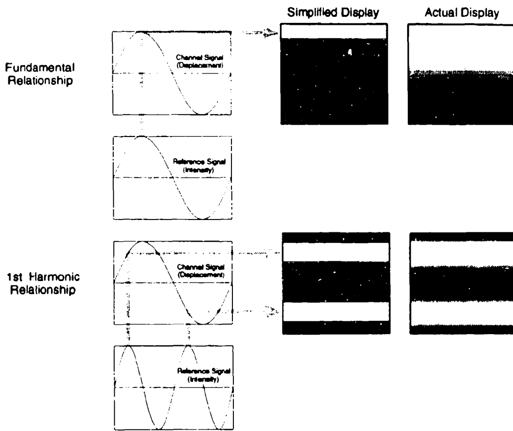
Figure 9. Expected Test Displays on the AFIT Toposcope. Input signals are sinusoids. The reference signal determines the brightness of the bar (only the peak brightness is shown in the simplified version) and the channel signal determines the vertical position of the bar within the box. Note the intensity gradients occurring in the actual display. Displays shown are not instantaneous but represent the composite display as seen by an observer.
