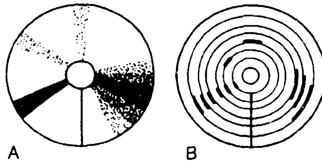
Figure 5. Comparison of Resolution of Original and Updated Walter-Shipton Displays. A . The photographically integrated original display is ambiguous when presented with short duration signals or those slightly offset from the frequency of interest. B . The circular display clarifies these ambiguities, showing brief signals in the 10 and 12 o'clock directions, a steady, harmonic signal at 8 o'clock, and a steady, but non-harmonic signal at 4 o'clock, resulting in a constant shift in subsequent traces (39:220).
