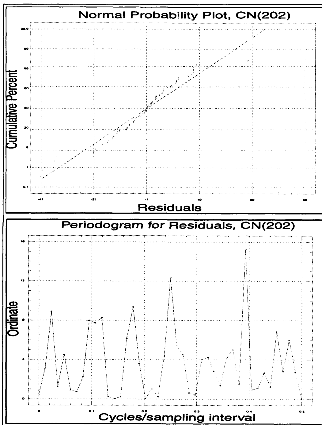
Figure F.88. Cumulative probability plots and periodograms for Model CN(2,0,2).
