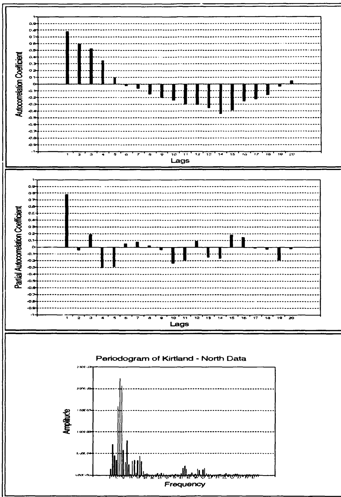
Figure F.13. ACF and PACF plots for the north azimuth at Kirtland AFB, New Mexico.
