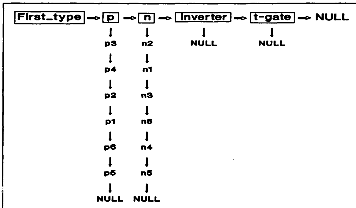
Figure 8. Example of Library and Component Linked Lists.
