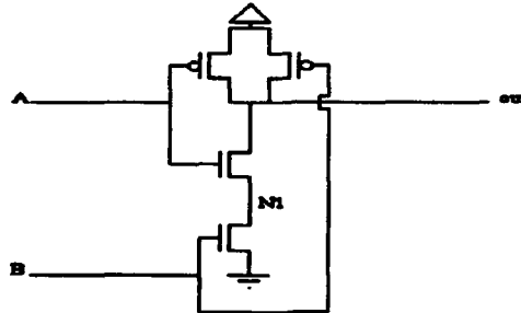
Figure 6. NAND Gate Template and Circuit.
