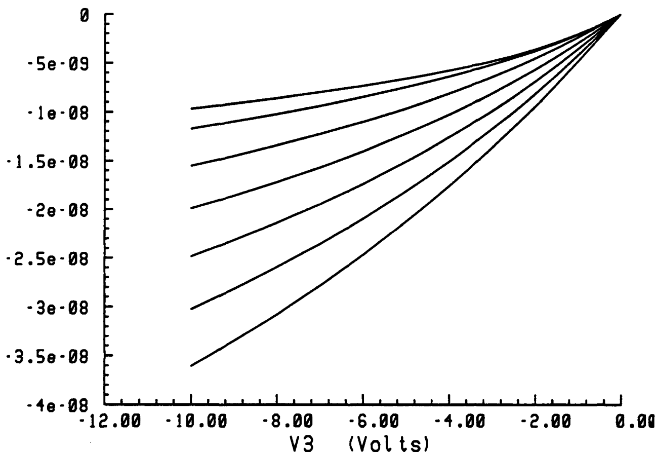
Figure 2. Drain Current versus Drain Voltage for the NOSC Device for V_g = 12 \text{ v} (top curve) to V_g = 0 \text{ v} (bottom curve) in Steps of -2 \text{ v} .
