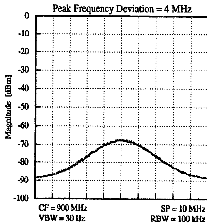
Figure 5-6 Spectrum Analyzer Displays of Two FM-by-Noise Barrages Modulated by 50 kHz Noise and Having Unequal Peak Frequency Deviations
