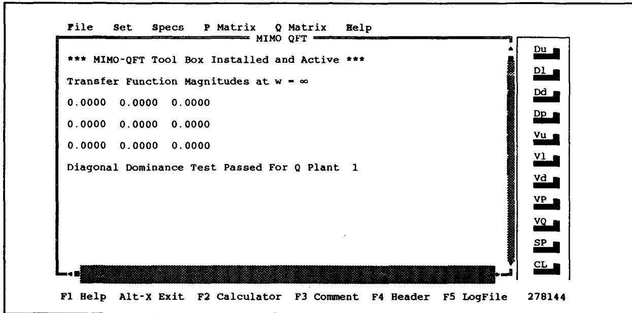
Fig. 5-9: Diagonal Dominance Check of Q Matrix Plant 1
