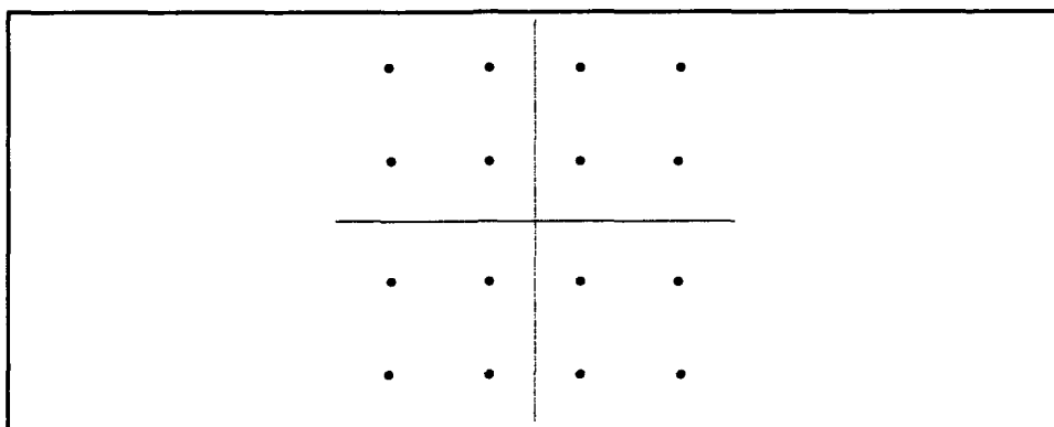
Figure 6. 16-QAM constellation
