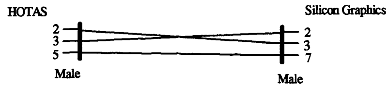
Figure 12. HOTAS to SG Cable Connections
