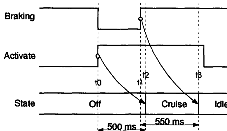
Figure 65. Braking During Activate Asserted Test Timing Diagram
