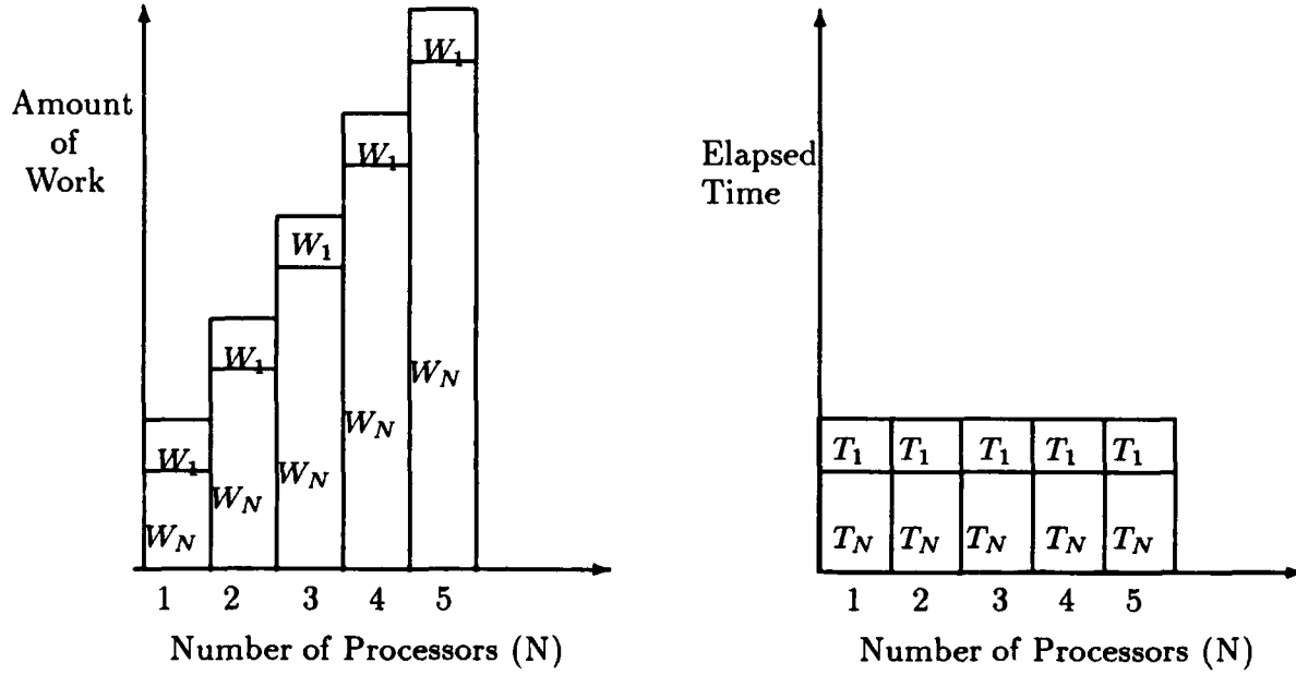
Figure 4. Gustafson's scaled speedup.
