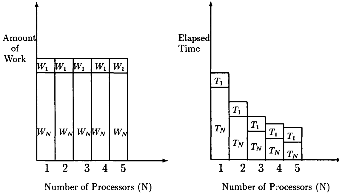
Figure 3. Amdahl's law.
