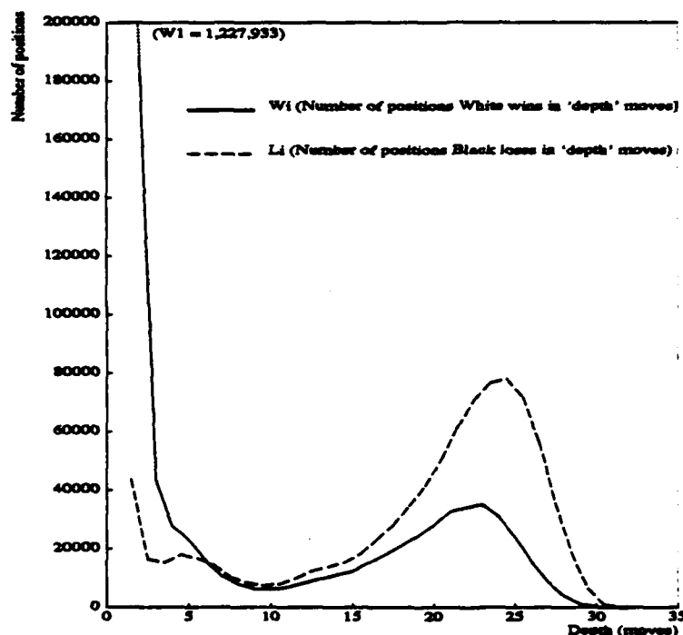
Figure 5.1: Distribution of depths, BTM and WTM, for KQKR
