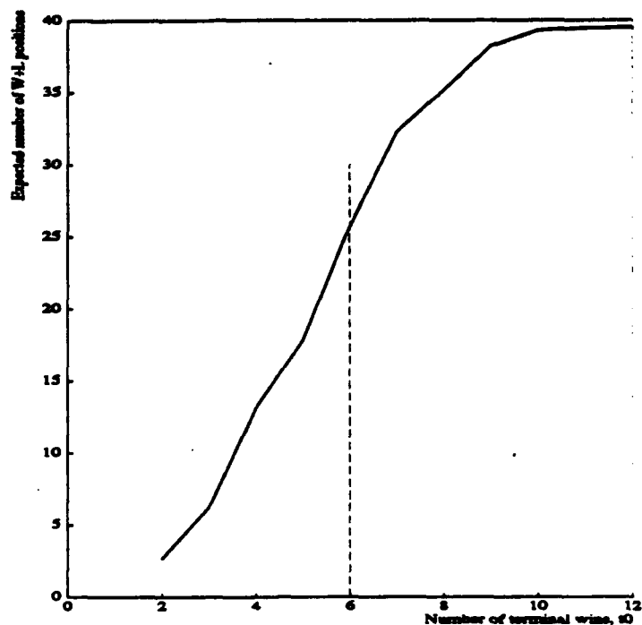
Figure 3.2: Expected number of winning positions in a game with b = 2 and N = 20 , as a function of t_0 .
