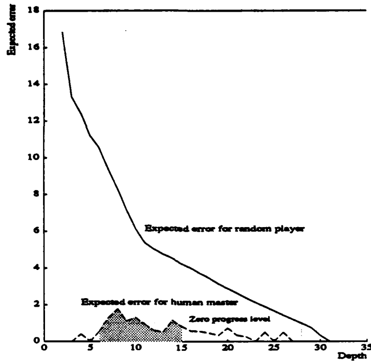
Figure 6.3: Expected error d for human masters, as compared to the random player.
