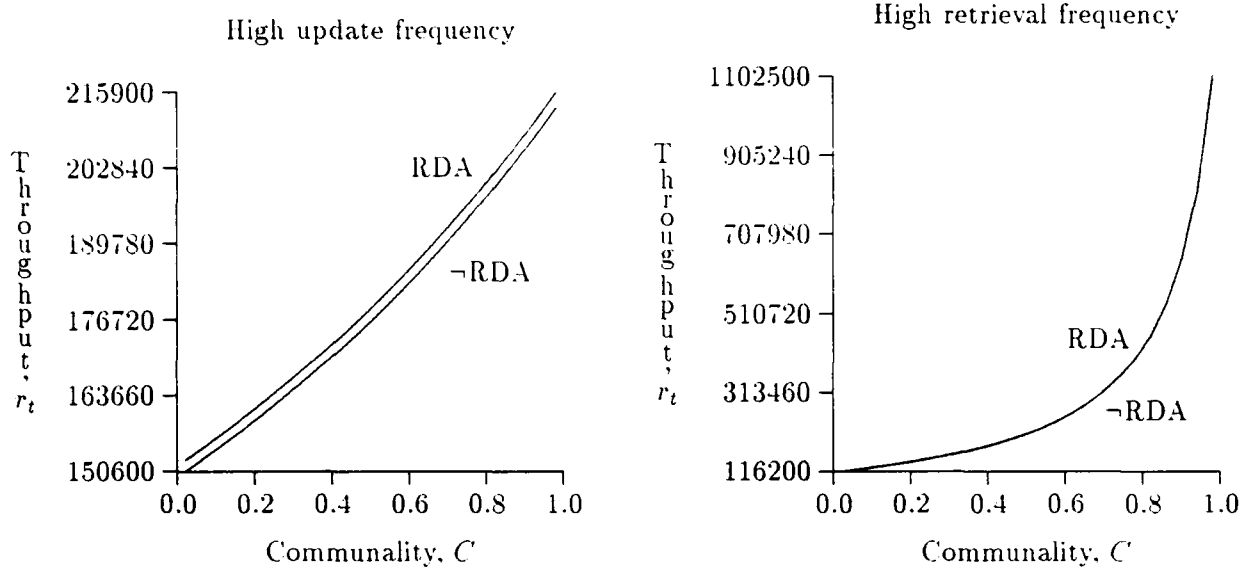
Figure 11: Results for \neg ATOMIC, STEAL, FORCE, TOC, in the case of record logging.
