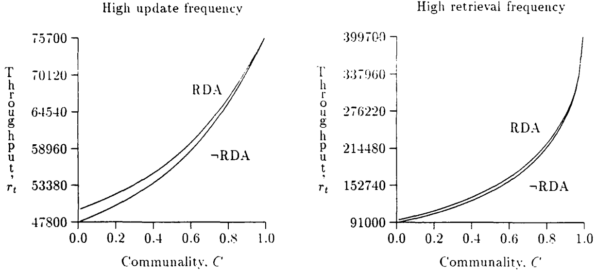
Figure 10: Results for \neg ATOMIC, STEAL, \neg FORCE, ACC
