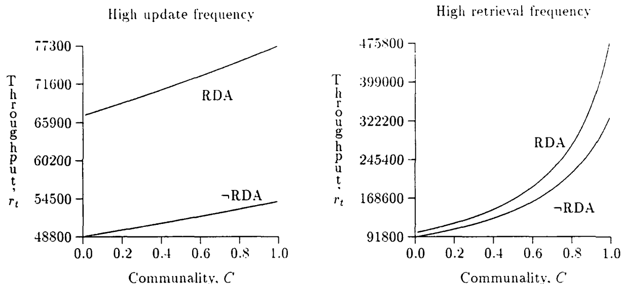
Figure 9: Results for \neg ATOMIC, STEAL, FORCE, TOC
