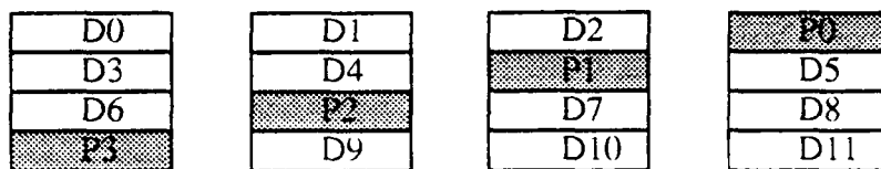
Figure 1: RAID with rotated parity on four disks.
