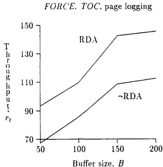
Figure 14: Empirical results for FORCE. TOC algorithms with page logging.
