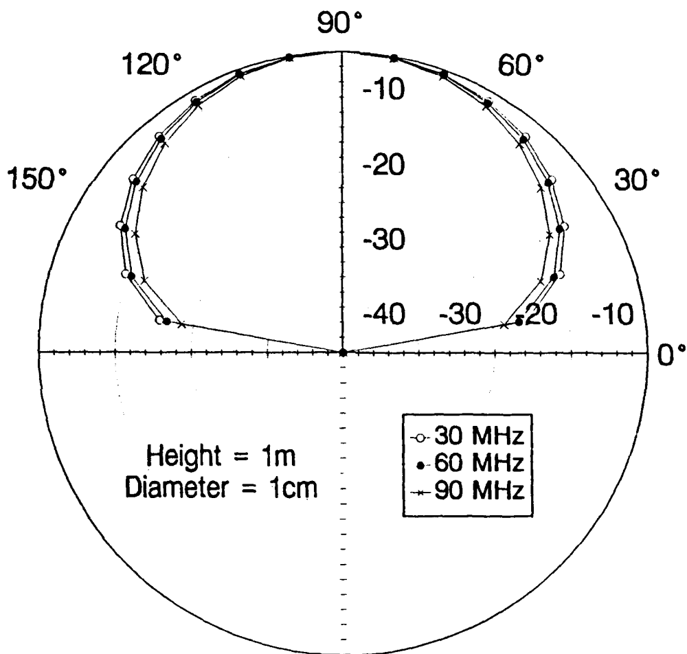
Radiation Pattern of Resistively Loaded Monopole
