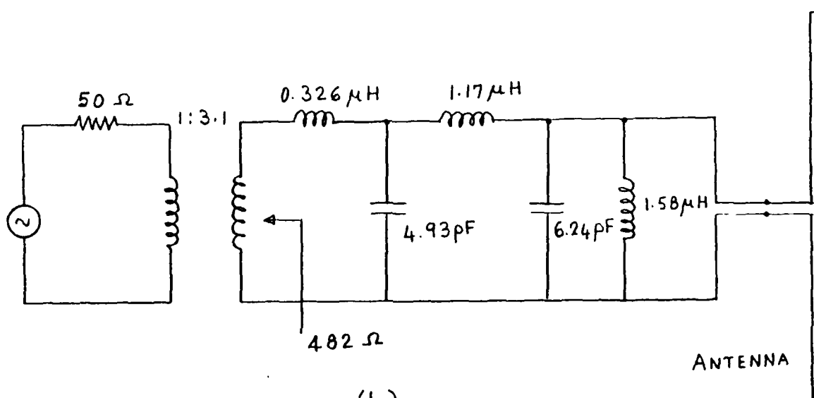
FIG. 6. CIRCUIT REALIZATIONS
