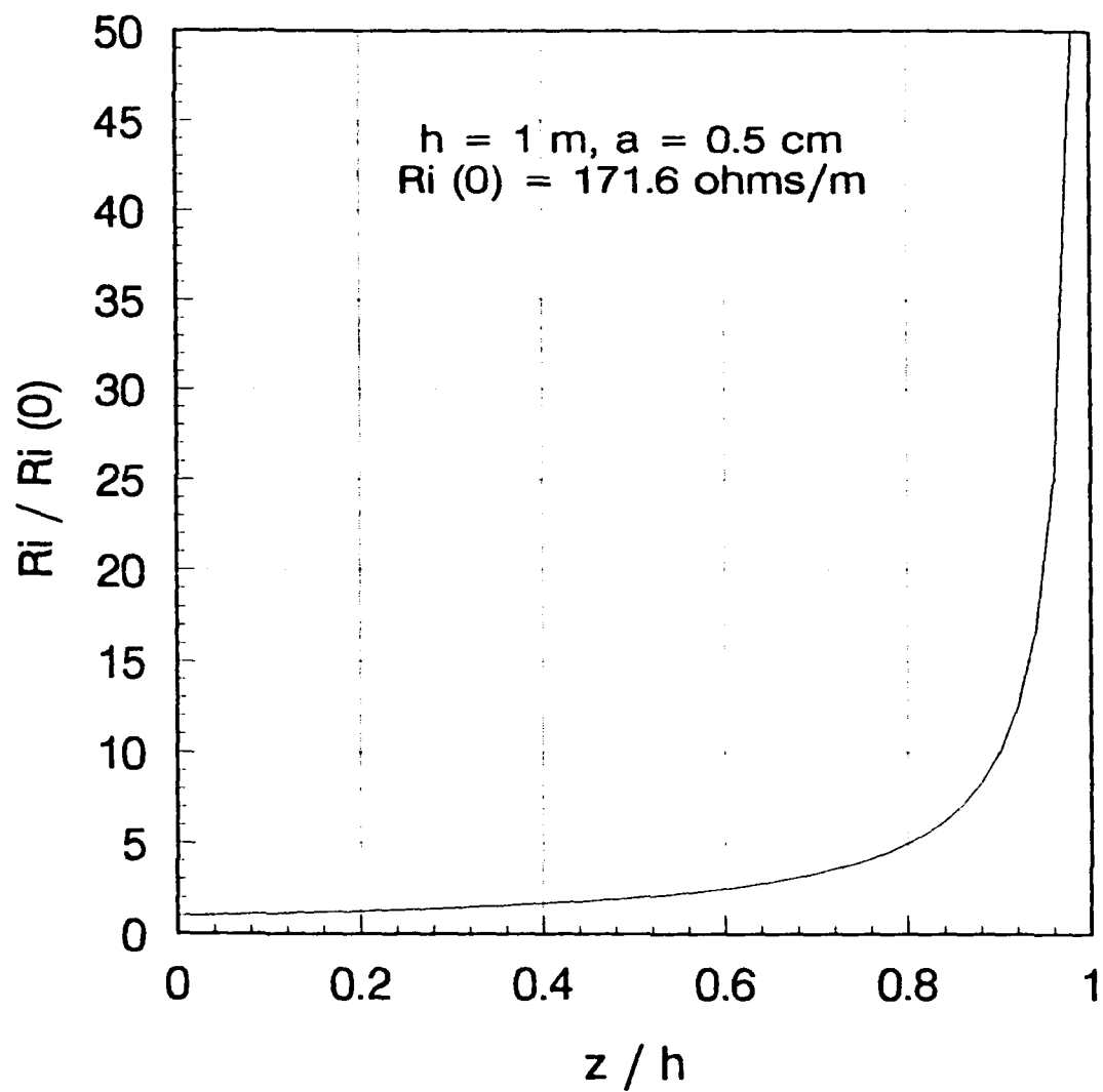
Fig. 1 Variation of Resistivity along Monopole
