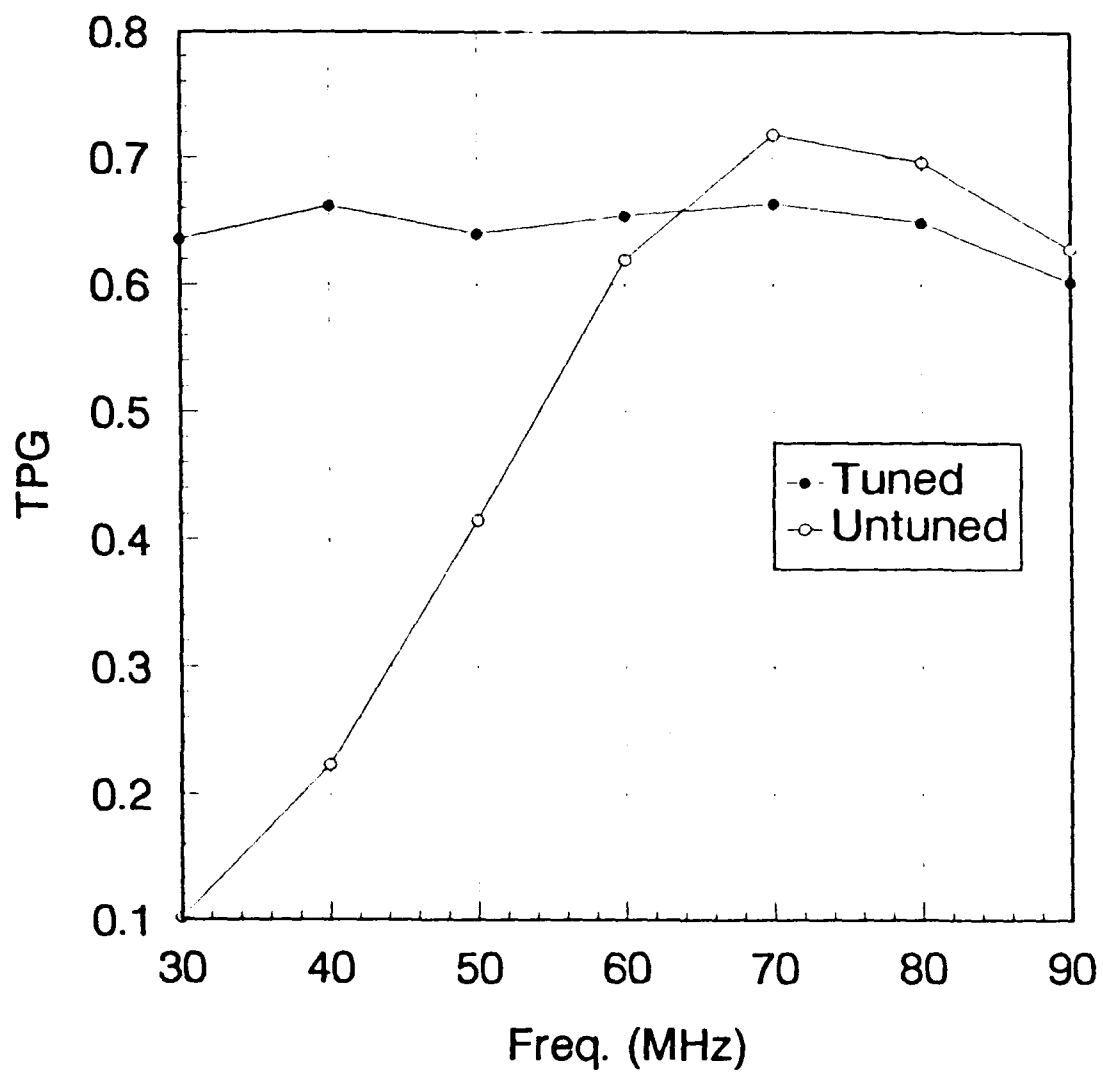
FIG. 7. TRANSDUCER POWER GAIN FOR RESISTIVELY LOADED MONOPOLE
