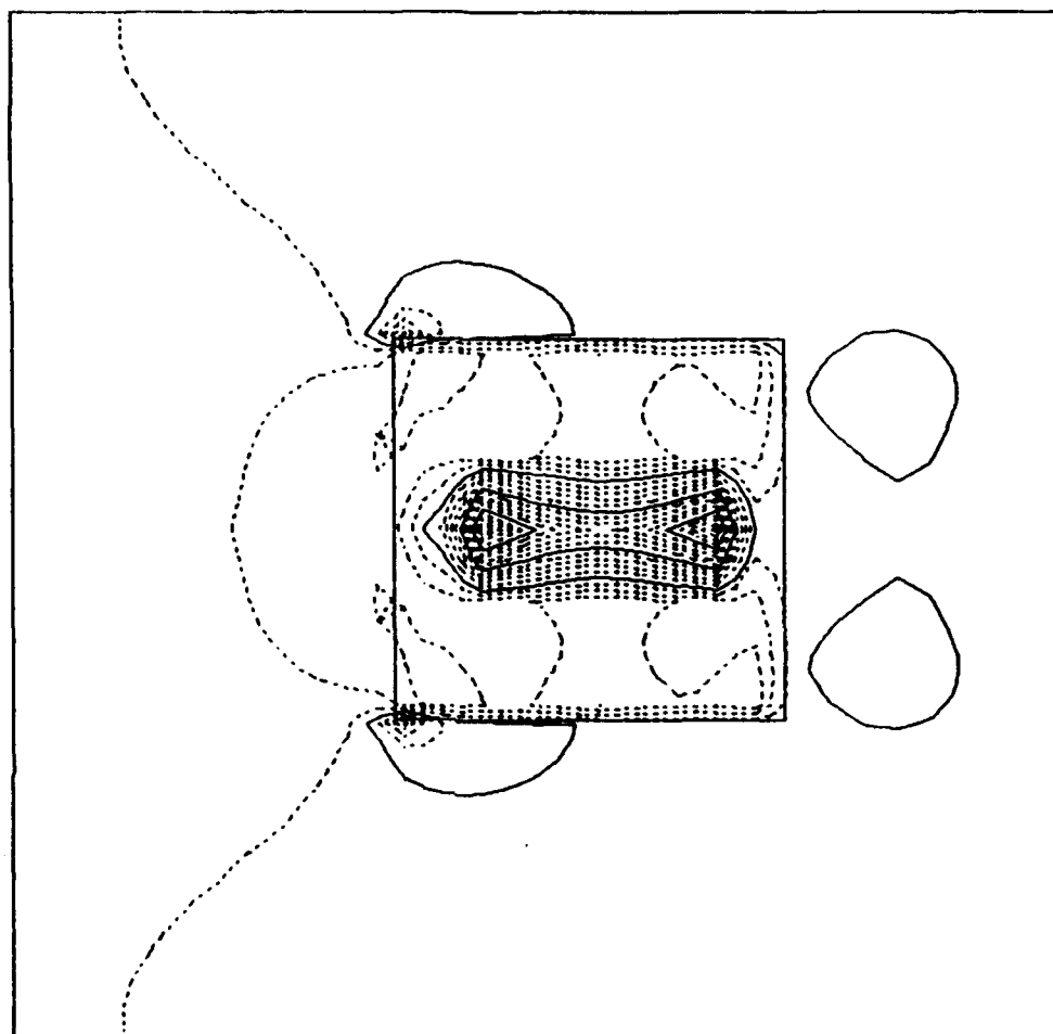
Figure 21. Pressure contours for the case in Figure 20.
