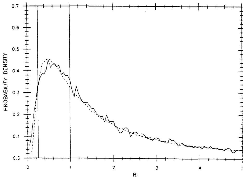
Figure 4.11: The randomly sampled Richardson number pdf for the FASINEX data (solid line) and the Desaubies and Gregg- N^2, \chi^2_2 - S^2 Richardson number model.
