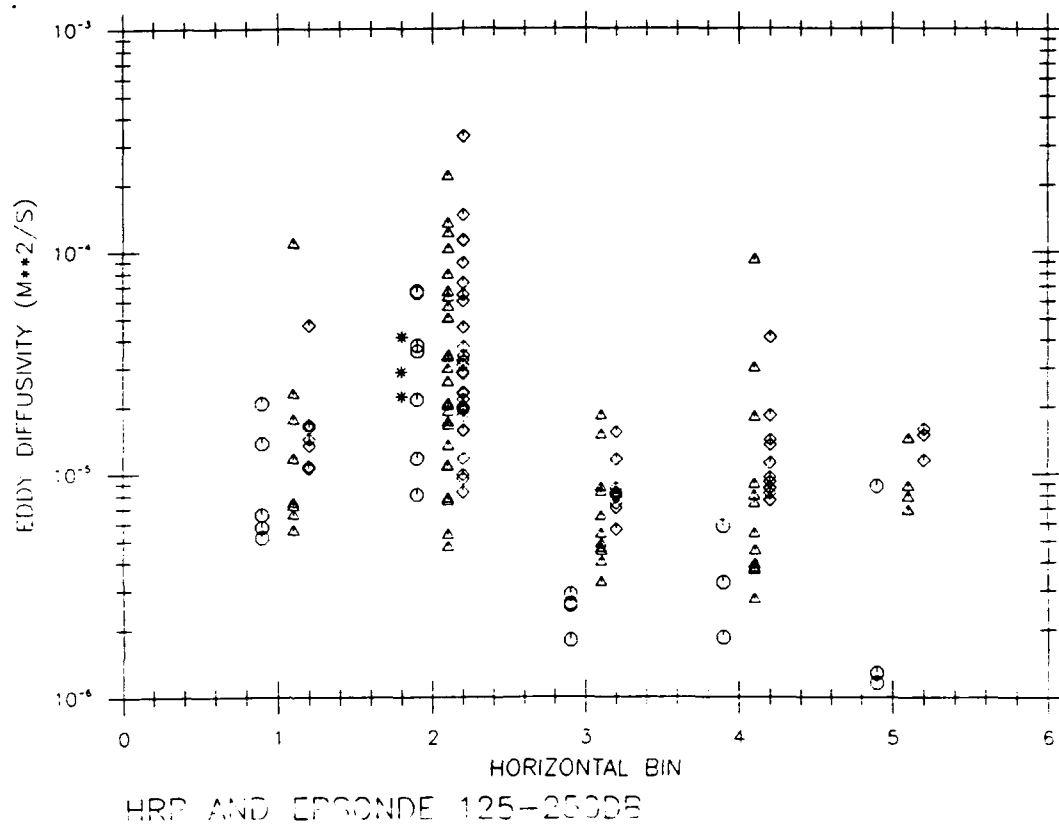
Fig. 2.11: Estimates of eddy diffusivity averaged over 125-250 m. for individual casts and plotted with respect to their position relative to the front. The symbol \circ denotes HRP K_T , * HRP K_p , \Delta EPSONDE K_T and \diamond EPSONDE K_p estimates. The various symbols are offset within each bin for clarity.
