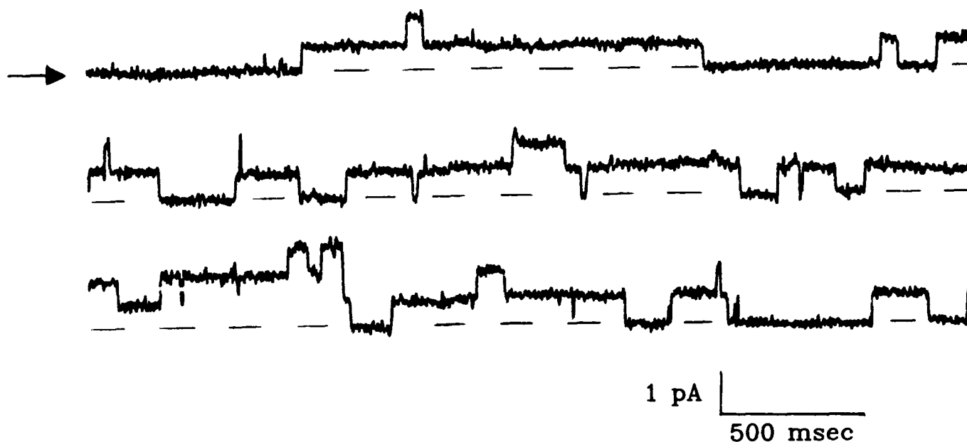
Fig. 1. Electrical activity from excised patch of freeze-thaw liposomes prepared with crude membrane fraction (i.e., whole Na + channel). Single-channel conductance was 10 pS when bathed in 150 mM NaCl; pipette voltage ( V_{\text{pipette}} ) = +60 mV. Arrows and dashed lines indicate current measured from quiescent membrane.
