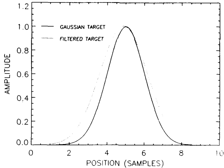
Fig. 20 — Effect of S4(1/4, 1/2) DDF with \sigma = 1.0 Gaussian constraint on a \sigma = 1.0 Gaussian target
