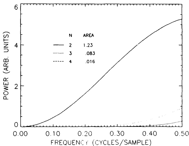
Fig. 11 — Error spectra for SLF-2, 3, and 4, and a p = 4 power law
