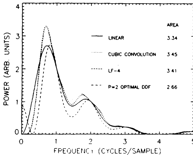
Fig. 4 — Error spectra |E_s(v) F(v)|^2 when the image spectrum is a p = 2 power law, for three interpolators and one DDF at the shift s = 0.25
