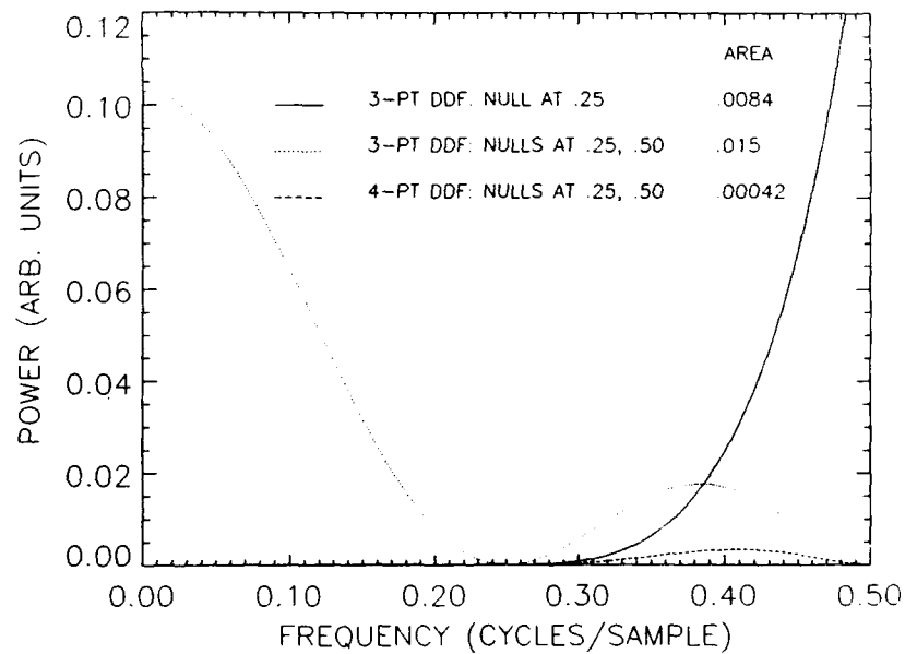
Fig. 15 — Error spectra for hybrid DDFs and a p = 2 input spectrum
