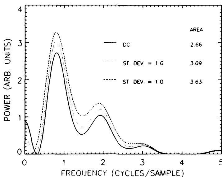
Fig. 6 — Error spectra after use of the optimal two-point DDFs, for three different filter constraints. The input signal spectrum is a p = 2 power law.
