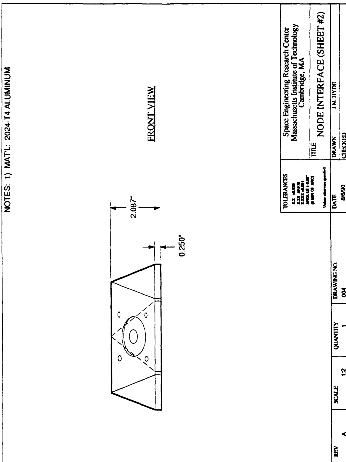
Figure A.3: Node/motor interface engineering drawing, sheet #2.
