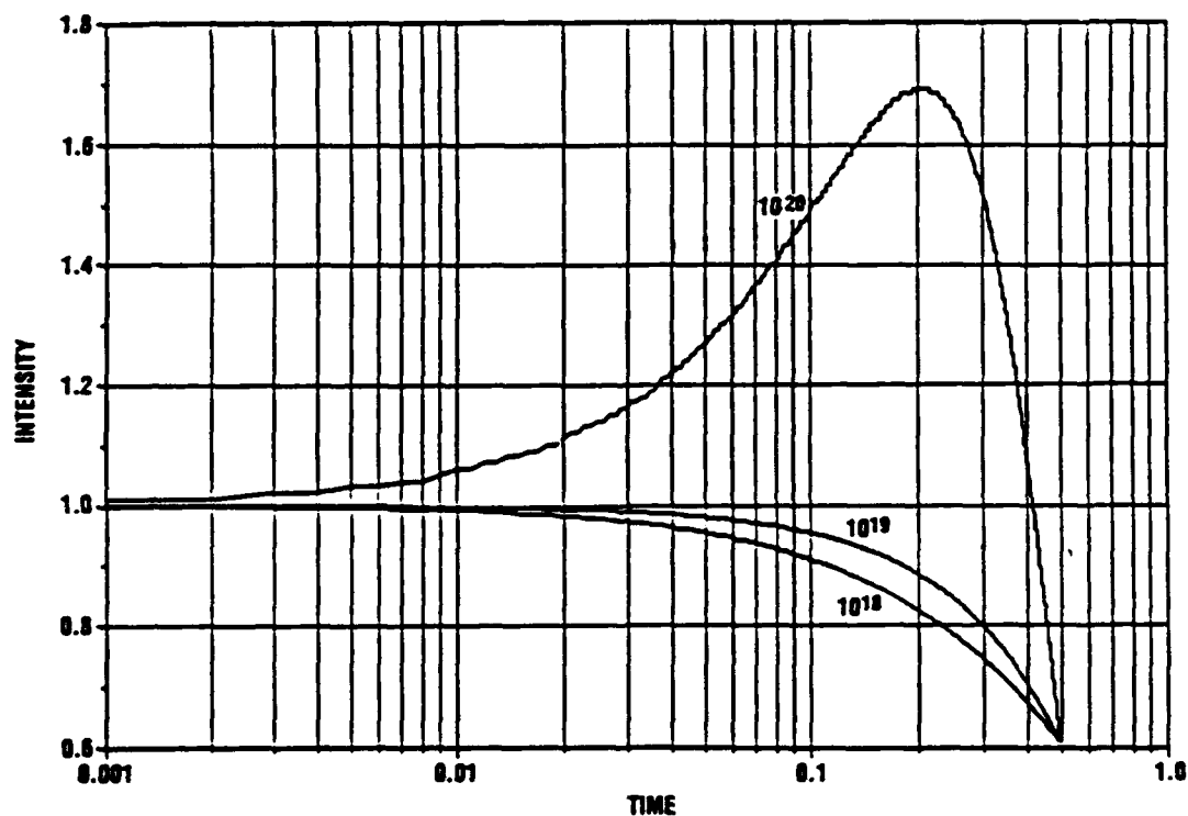
Figure A-2b. Plot of the ASE pulses for values of the initial inversion density in the threshold region between \rho = 10^{19} and \rho = 10^{20} \text{ cm}^{-3} .
