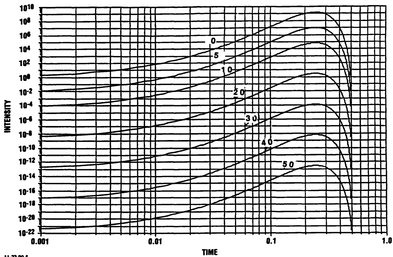
Figure A-3. Logarithmic plot of the ASE pulses for g = 1 , \rho = 10^{22} and different values of the attenuation coefficient \mu as indicated on graph.
