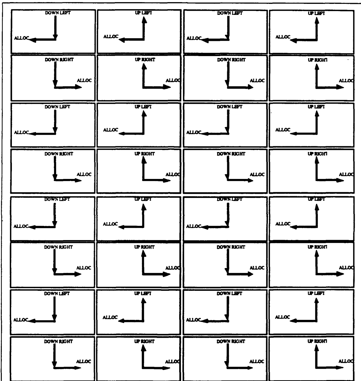
Figure 5-9: The central crosspoint switching array.
