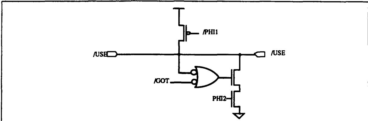
Figure 5-18: The dynamic wired OR structure of the crosspoint column USE signal.
