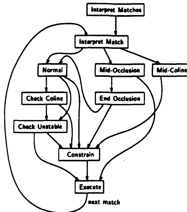
Figure 3.3: A block diagram of the interpretation process at each node in the search tree.
