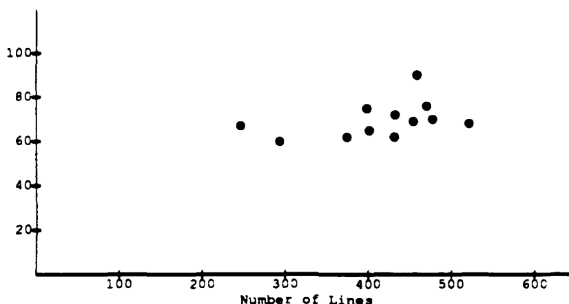
Figure 2.14: The number of groups (with four or more members) found in an image, plotted against the number of lines (of length greater than eight pixels) in the image.
