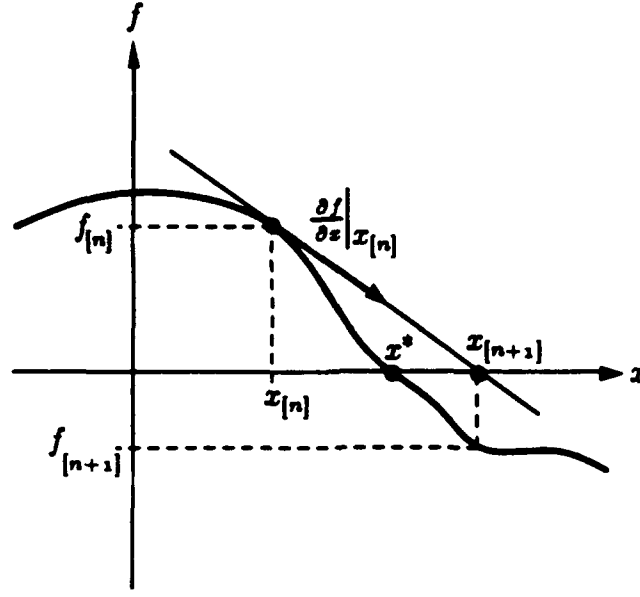
Figure 5.2: A single iteration in Newton's method for solving one equation in one variable.
