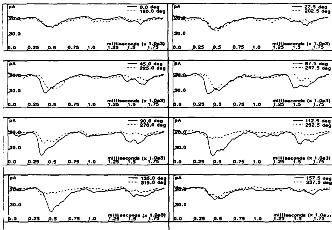
Figure 3.5: DS responses to moving grating under voltage clamp for cell A47 (protocol A47WF15), taken 2 hours after the responses in Figure 3.3. Holding potential = -80mV, average of 4 trials. Stimuli are identical to those used for Figure 3.3. Using the integral of (I_{holding} - I_{clamp}) as the response variable, the DS statistics are \theta_P = 112.5^\circ , DI_{sum} = 0.3 ( p < 0.05 ). The preferred direction has apparently shifted from the previous protocol (though the statistical significance of this was not evaluated), but remains consistent with the original axis of asymmetry.
