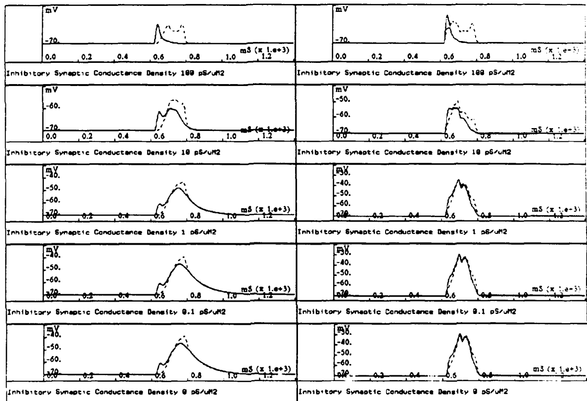
Figure 4.9: Example set of simulations for cell in Figure 4.8 for a stimulus moving at 4 \mu\text{m}/\text{msec} at various values for G_{in} and C_m . On the left C_m = 1.0 \mu\text{F}/\text{cm}^2 , and on the right C_m = 1.0^{-5} \mu\text{F}/\text{cm}^2 . Tip output is from the righthand distal tip in Figure 4.8, and the solid and dashed waveforms are for leftward and rightward motion, respectively. When inhibition is absent (bottom simulations) the cable capacitance distorts the equal area waveforms so that a nonlinear integrator may distinguish them (bottom left). If the nonlinearity saturates, then the "fatter" leftward response yields a larger total output than the higher amplitude rightward response (DS reversal). With no inhibition and very low capacitance (bottom right) the waveforms become mirror-symmetric.
