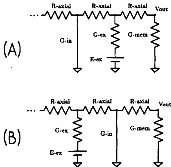
Figure 4.4: The effect of inhibition on output is dependent on the relative positions of the excitation and inhibition with respect to the output. To illustrate, we use an extreme case in which the inhibitory battery is equal to the resting potential, and the activated inhibitory conductance is infinite. In (A) the excitatory input is closer to the tip than the inhibitory input. Although the membrane potential at the site of inhibition is clamped to the resting potential (short-circuited), the axial resistance of the cable partially isolates the excitatory location, and the tip ( V_{\text{out}} ) is depolarized. In (B) the interposed inhibitory input clamps the cable between the excitatory input and the output to the resting potential, so that the output stays at rest. Adding membrane capacitance, a finite conductance to the activated inhibitory synapse, or making the inhibitory reversal potential not exactly equal to the resting potential does not change the basic interaction. However, a non-zero R_{\text{axial}} is crucial.
