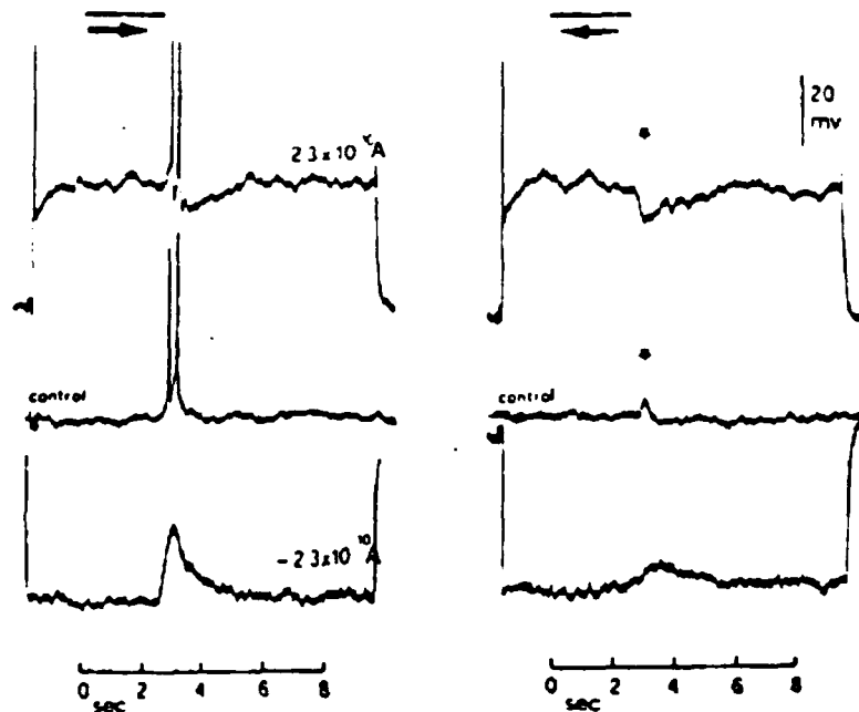
Fig. 8. The effect of intracellular current injection upon the photoresponses to a moving spot. The trajectory of the spot ( 991 \mu\text{m} at 3.5 \mu\text{m}/\text{msec} ) was along the preferred-null axis. The responses to movement in the preferred and null directions (marked by a star) are shown at the left and the right side of figure, respectively. At the top, the duration and the direction of movement are indicated. Control indicates responses recorded at resting potential. Upper and lower records show the photoresponses during artificial polarization of the cell membrane obtained with the current intensity indicated by the numbers above the records on the left. Zero time coincides with the onset of the spot movement.
