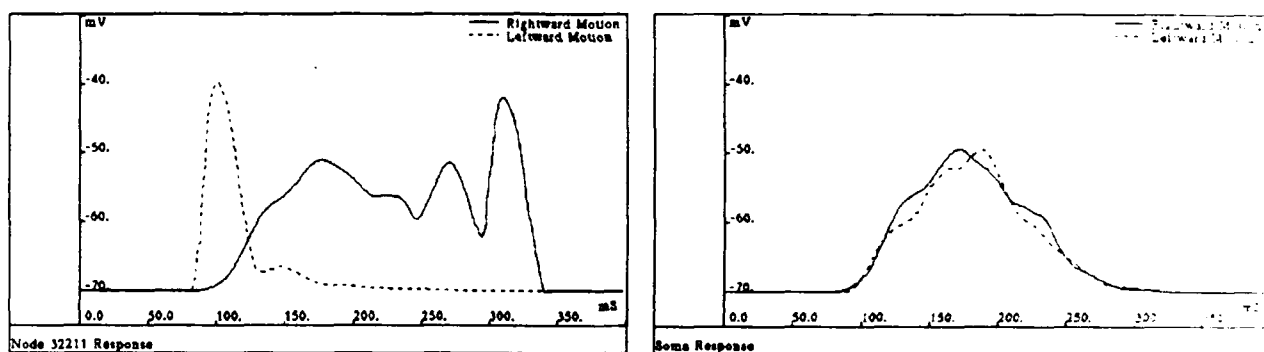
Figure 4.6: Responses of cell in Figure 4.5 to 50\mu\text{m} slit moving from left to right and back again at 2\mu\text{m/ms} . The voltage at the rightmost distal tip in Figure 4.5 (Node 32211) is highly DS, whereas the soma response is barely DD. Model parameters are given in the text. Simulations also show that inclusion of a K^+ conductance which inactivates with depolarization can both facilitate the preferred-direction response and attenuate the null-direction response (see Sections 4.1.5 and 4.3.3).
