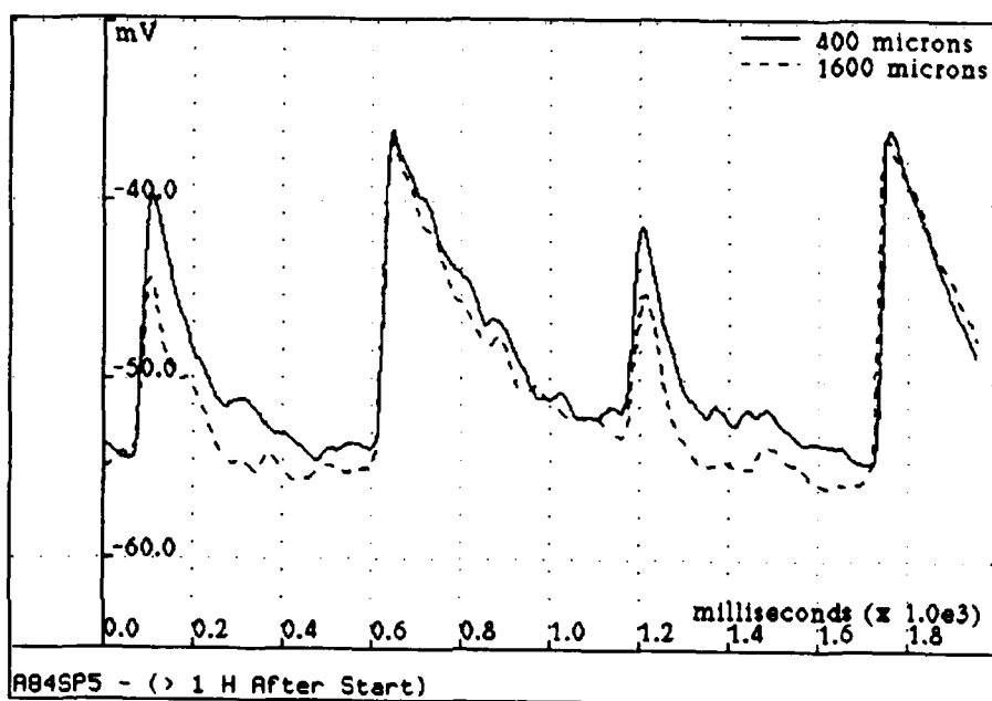
Figure B.8: Response of cell AR1, taken more than one hour after start of whole-cell access (average of 4 trials). E_{rest} = -55 mV. This cell now show an ON/OFF response, and each edge response is simpler than the initial recording. These responses suggests that inhibitory input to the cell has been blocked, uncovering an underlying excitatory ON/OFF input. Actual blockage of inhibitory synaptic channels is further supported by the slight rise in E_{rest} ( \approx 5 mV), although, as mentioned earlier, it was more typical to see a drop in E_{rest} over time. Note also the loss of antagonistic center/surround properties in this particular cell. As noted in the text and in Figures B.10 to B.12, in many cells a loss of IPSPs was seen over time with nonetheless maintenance of center/surround properties. As before, on/off/on/off transitions of light spot are at 0, 500, 1000 and 1500 ms, respectively.
