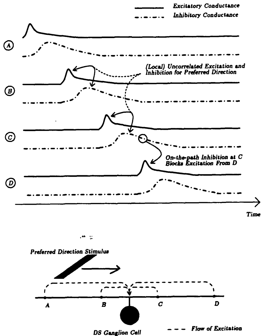
Figure 2.6: DS models in which the ganglion cell dendritic tree is the site for DS excitatory-inhibitory interactions (correlation of local inputs in the null direction) predict inhibition of the late phase of long distance preferred direction motion and subunit preferred response that depends on location, assuming that inputs occur throughout the tree. This inhibition is from previously activated inhibition (e.g. at C ) that is non-correlated with local excitation, but that is nonetheless both on-the-path and correlated for the later excitation (e.g. at D ).
