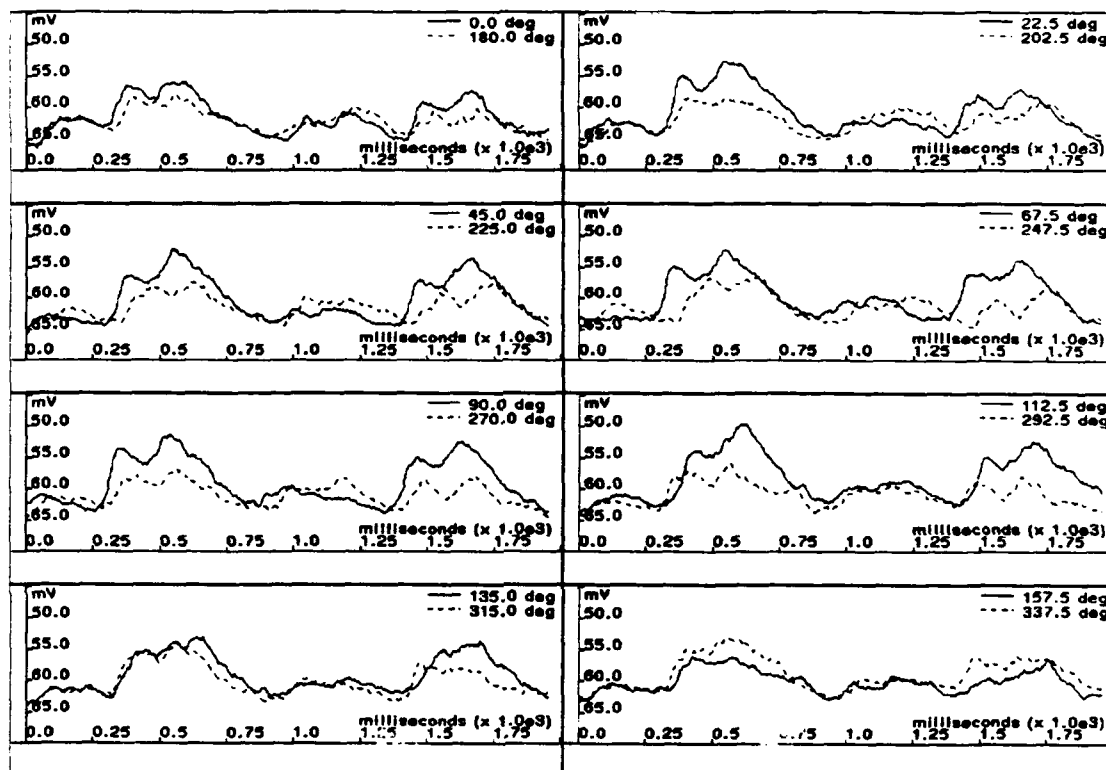
Figure 3.3: DS responses to moving gratings under current clamp for ON/OFF ganglion cell A47 (protocol A47WF3). Each waveform is the average of 4 trials. The grating had a 200\ \mu\text{m} square aperture, a temporal frequency of 1 hz and a spatial period of 800\ \mu\text{m} . In this protocol, \theta_p = 67.5^\circ , DI_{sum} = 0.2 ( p < 0.05 ) (integral of V - E_{rest} ). This recording was made 17 minutes after whole-cell access (there was no extracellular response recorded). Although this cell responded to both ON and OFF edges of stationary spots, the expected 2nd harmonic of the motion response is small. Small IPSPs were observed within 5 minutes of whole-cell access during receptive field stationary spot mapping.
