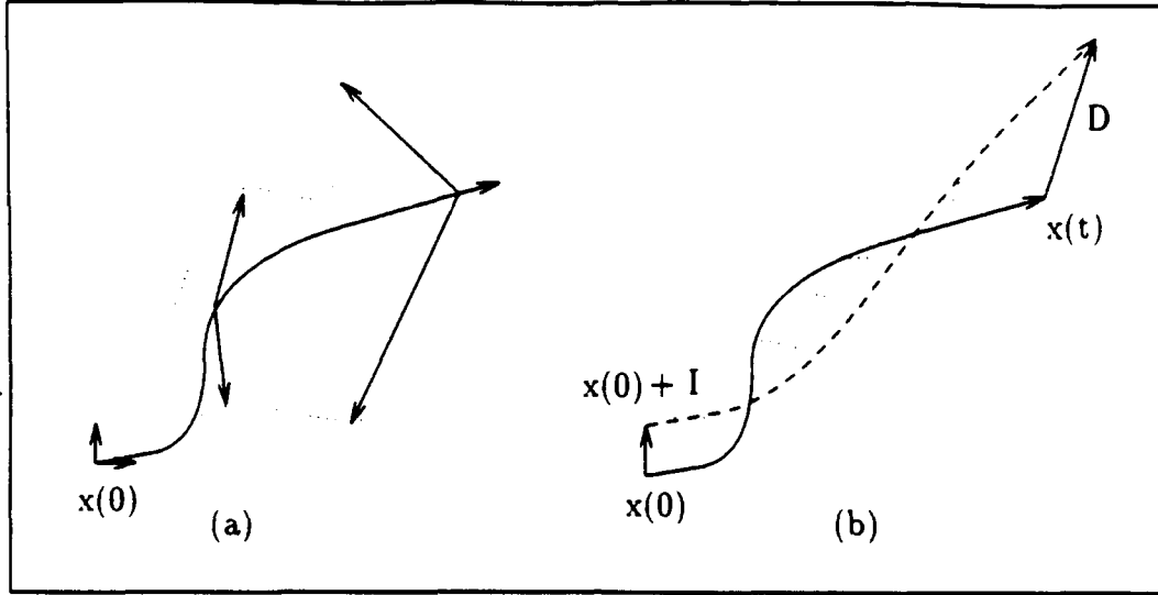
Figure 5.13: The geometry of the variational system: (a) the evolution of the variational system (b) system trajectories from [\bar{x}_0] and [\bar{x}_0 + \bar{I}]
