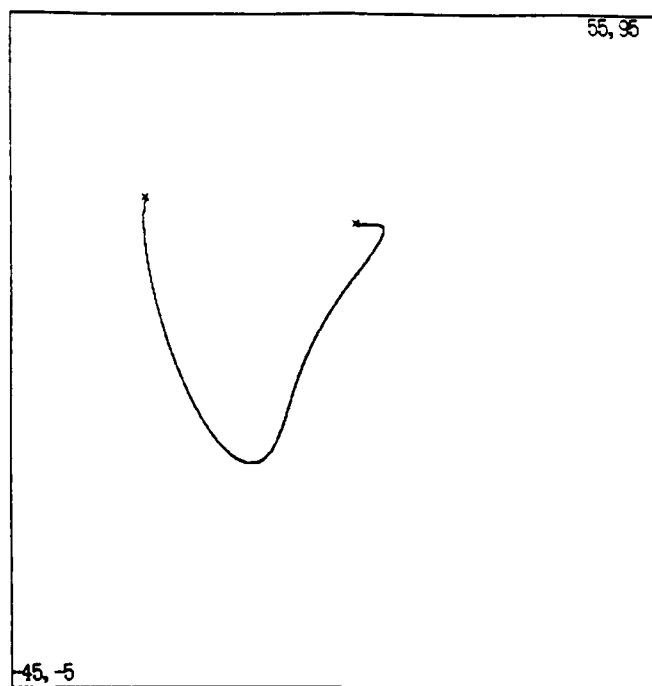
Figure 7.14: Numerical integration of segmented path
