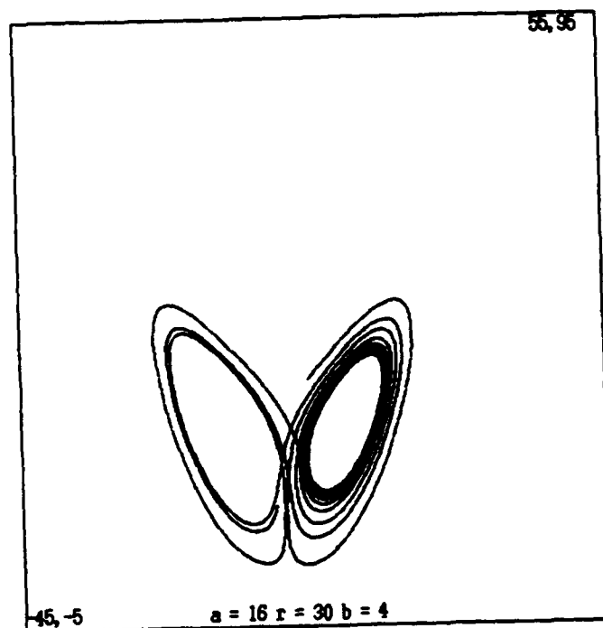
Figure 7.9: Lorenz attractor for r = 30
