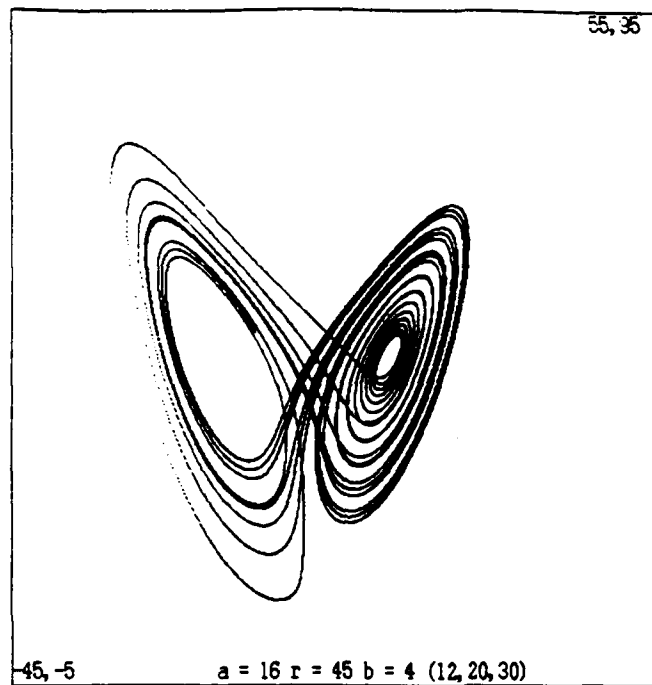
Figure 7.1: Lorenz attractor for a = 16 , r = 45 , and b = 4
