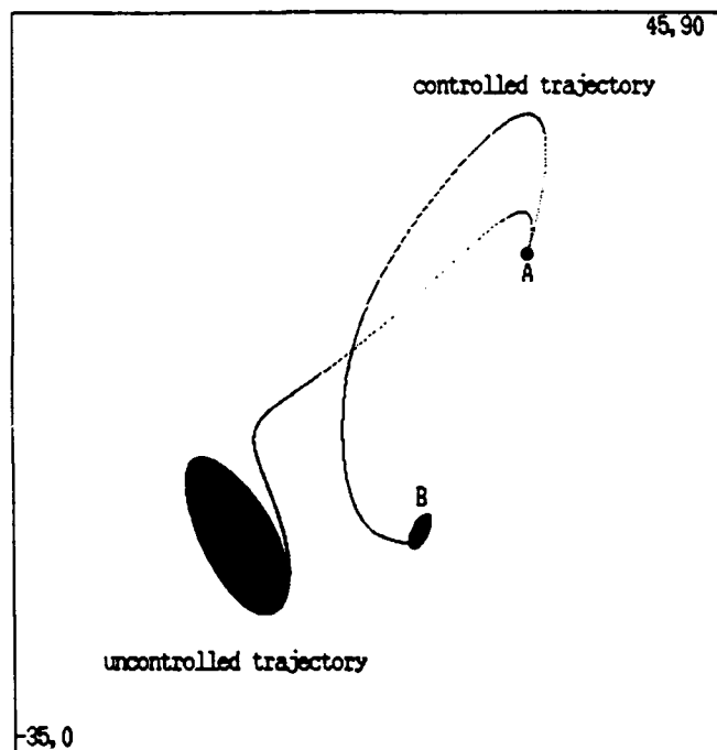
Figure 7.15: Segmented path to a fixed point
