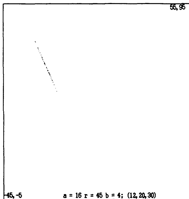
Figure 7.2: x - z section at y = -15 of Lorenz attractor for a = 16 , r = 45 and b = 4
