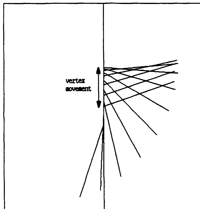
Figure 7.17: Movement of driven-vertex pendulum (twelve time-lapse images starting at (t, \theta, \omega) = (0, 1.9, 0) )
