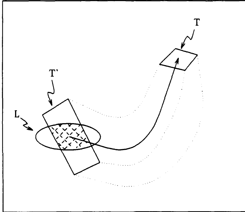
Figure 5.17: Computing whether a single-segment path meets a tolerance. The solid arrow is the path segment \tilde{S} ; T is the tolerance region at its endpoint. T' is the same region, integrated backwards to the starting point \tilde{S}_{init} . L is the domain of the junction controller at \tilde{S}_{init} . If \tilde{S}_{final} lies in T and \tilde{S}_{init} lies in the intersection of T' and L , the segment passes the check.
