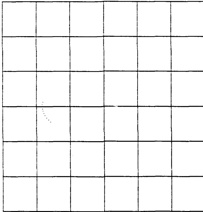
Figure 4.3: Discretizing a trajectory: this ten-point state-space trajectory \phi_i(t) starts at the point (-.785 -4.167) , the center of the grid cell \#(1 \ 2) . The discretized version of this trajectory, \Phi(z) , is ((\#(1 \ 2) \ .01) (\#(1 \ 3) \ .09)) . Region corners are (-\pi/2, -25) , (\pi/2, 25) and m = 6 .
