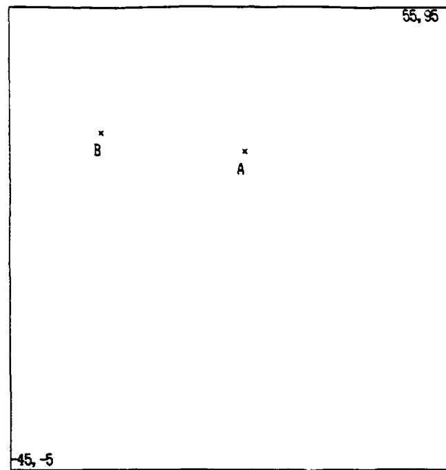
Figure 7.6: Origin and destination points
