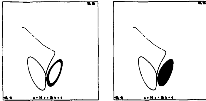
Figure 7.8: A “fixed point” for a = 16 , r = 25 and b = 4 : (a) ten orbits (b) 50 orbits
