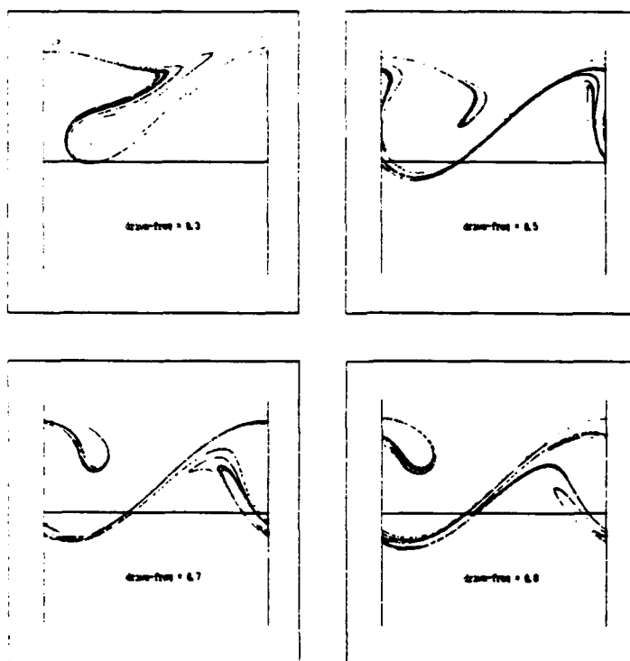
Figure 7.34: Chaotic phase-locked loop attractors at various drive frequencies
