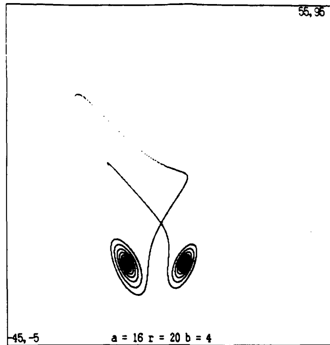
Figure 7.5: Two stable fixed points
