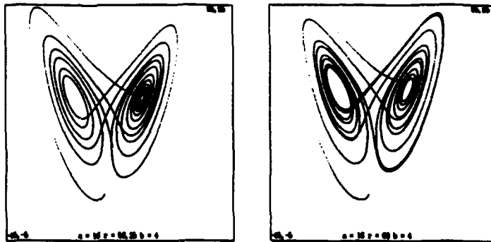
Figure 7.11: Lorenz attractors for r = 56.25 and r = 60
