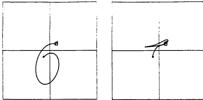
Figure 2.12: Perfect Moment's simulation of the controlled trajectory found for the Rössler example: the left-hand plot is an x - y projection and the right-hand plot is an x - z projection
