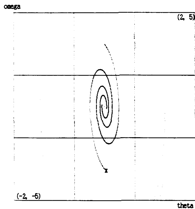
Figure 2.5: A state-space portrait of the damped pendulum with a 3 \times 3 grid. The horizontal axis is the angular position \theta and the vertical axis is the angular velocity \omega . Perfect Moment generates one trajectory from each cell, discretizes them into lists of cells touched, and synthesizes a rough dynamics classification for each
