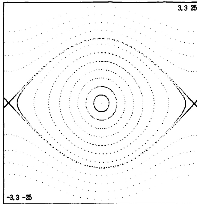
Figure 7.18: State-space portrait of the simple pendulum
