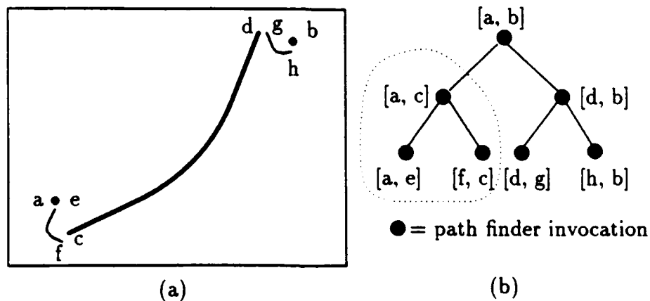
Figure 5.3: A segmented path (a) and the path finder calls that created it (b). [x, y] denote pairs of points to be connected at each pass; later calls are lower down in the tree and connect closer pairs
