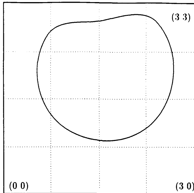
Figure 4.5: A period-one limit cycle
