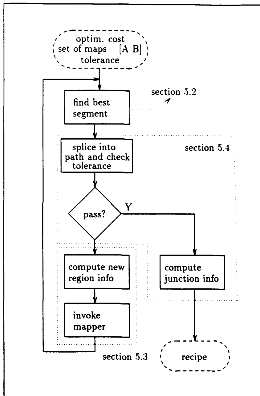
Figure 5.1: The path finder's flowchart: dotted boundaries group the topics according to the section where they are discussed
