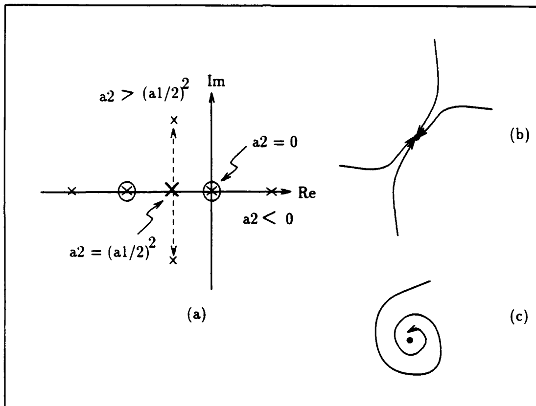
Figure 3.3: Pole selection for linear feedback control: (a) root-locus plot as a function of a_2 (b) overdamped behavior (c) underdamped behavior.
