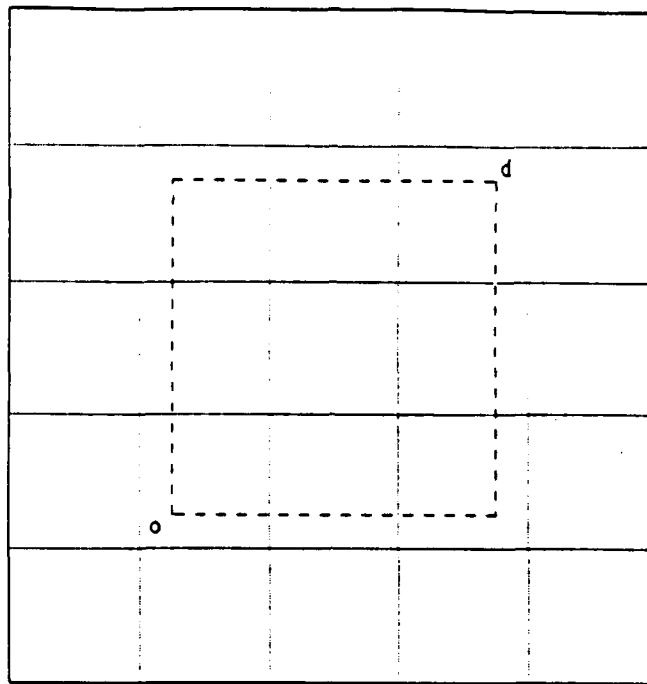
Figure 5.7: Initial search region and discretization with R = 2 and m = 5 . The bounding box of the origin (o) and the destination (d) is expanded by a factor of two along all state-space axes and each axis is divided into five intervals
