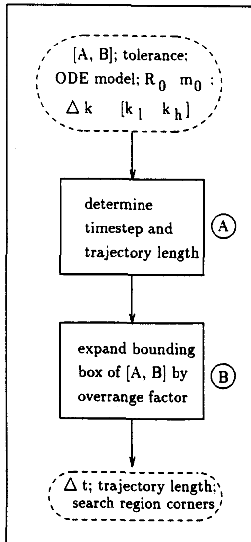
Figure 5.9: The initial operations required to set up the core segment search
