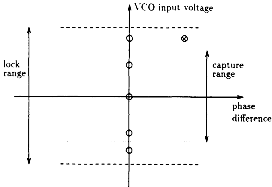
Figure 7.32: Lock and capture ranges
