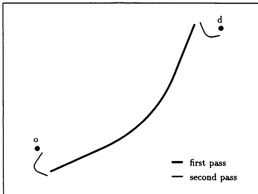
Figure 2.7: Schematic of a partial path after two passes: the core segment — found on the first pass — bridges most of the gap between the state-space points that are to be connected. Successive passes search for shorter segments that span the gaps in the path
