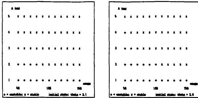
Figure 7.23: Stability of the inverted point via parametric resonance: \times = stable, o = unstable. Drive amplitude ( A ) versus drive frequency ( \omega ). (a) \theta_{init} = 3.1 (b) \theta_{init} = 2.9
