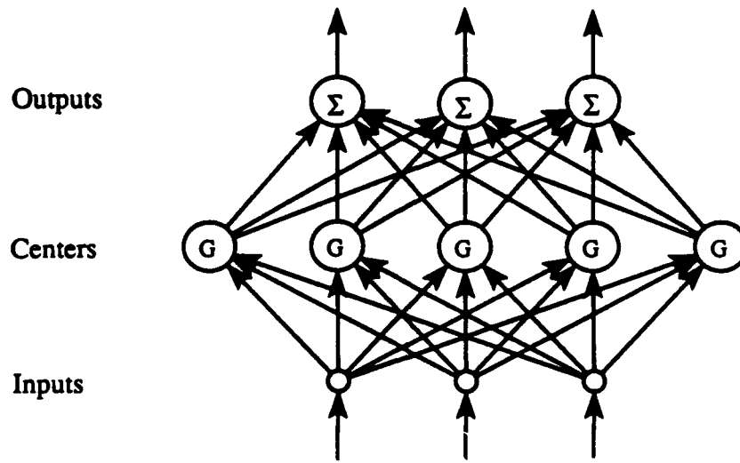
Figure 2.2: Typical radial basis function network with activation function G
