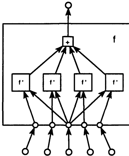
Figure 7.11: This figure is analogous to figure 7.6 and shows how f was split into four identical GRBF networks, f' , to be used in the recurrent network for learning two-dimensional segmentation. The outputs of each copy of f' are summed to produce the output for f .
