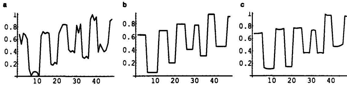
Figure 7.9: Input vector obtained by combining three length 16 vectors which the recurrent network was not trained on. b) Target output vector. c) Output of the recurrent network after iterating for eight time steps.
