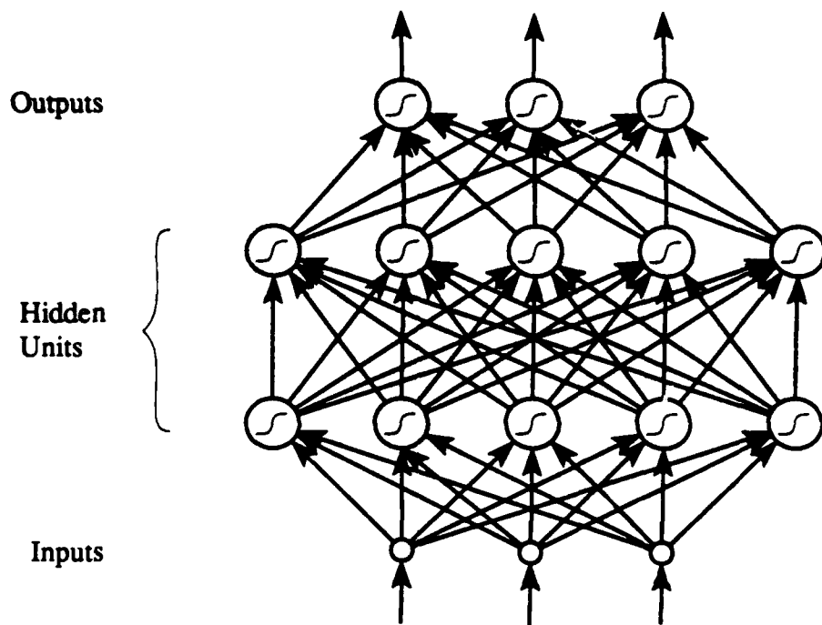
Figure 2.1: Typical sigmoidal network
