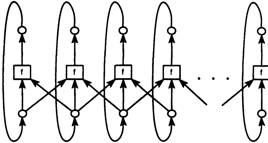
Figure 2.4: Recurrent network for dimensionality reduction. Each box contains a function f which is actually a feedforward network.
