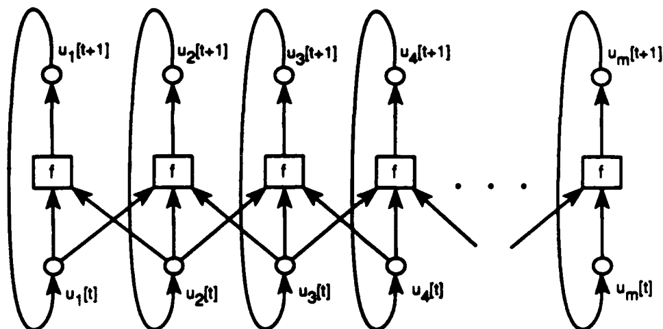
Figure 5.1: Recurrent network for dimensionality reduction. Each box contains a function f which is actually a feedforward network.
