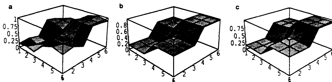
Figure 7.15: a) Input image used in training the recurrent network. b) Target output image. c) Output of the recurrent network trained to learn two-dimensional segmentation. The network was iterated for ten time steps.
