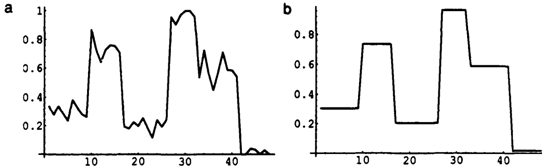
Figure 7.2: Typical training pair for the one-dimensional segmentation problem. Figure (a) is the input vector and (b) is the output obtained by running Hurlbert's segmentation algorithm on the input.
