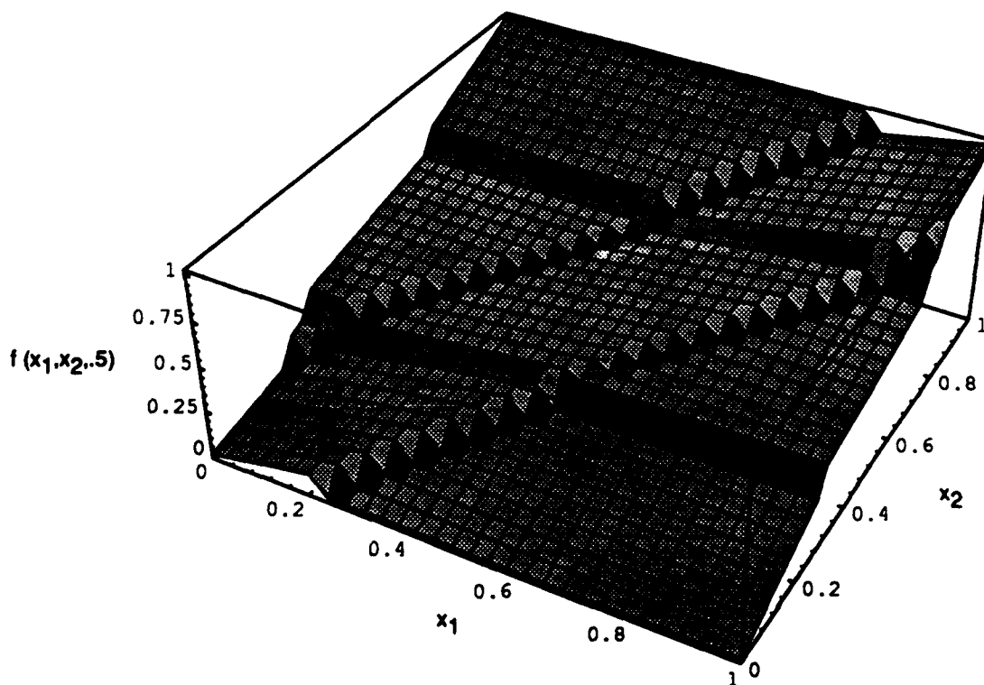
Figure 7.4: A slice of the graph of f(x_1, x_2, x_3) as defined in equation 7.2 with x_3 = 0.5 .
