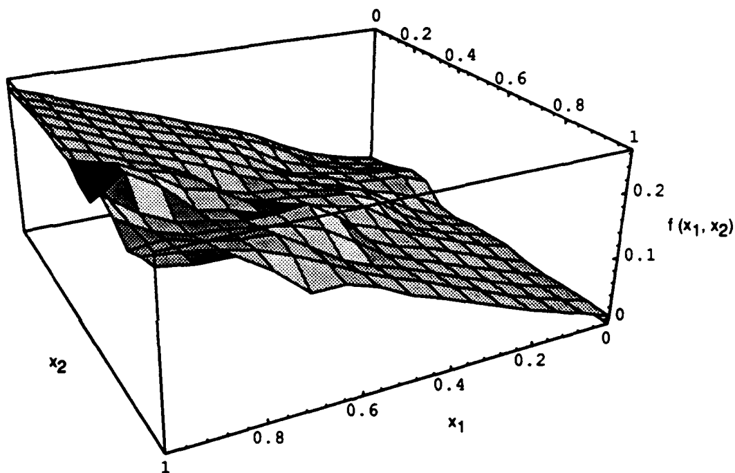
Figure 7.14: Graph of the function f' learned by the recurrent network.
