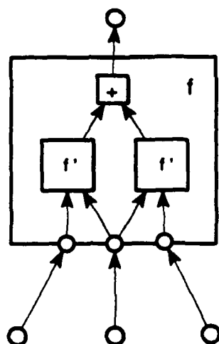
Figure 7.6: This figure shows how f was split into two identical GRBF networks, f' , by taking advantage of the symmetry of the image segmentation mapping. The f' boxes contain the same GRBF network; only the inputs differ. The outputs of each f' are summed together to produce the output for f . This construction is used by the recurrent network of figure 7.3.
