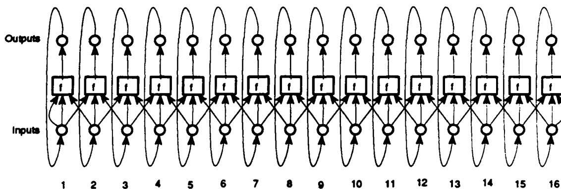
Figure 7.3: This recurrent network was used to learn the one-dimensional segmentation mapping in which the input and output images were 16 pixels long. Each box represents a copy of the same GRBF network which takes a neighborhood of pixels as input and outputs the value of the middle pixel on the next time step.
