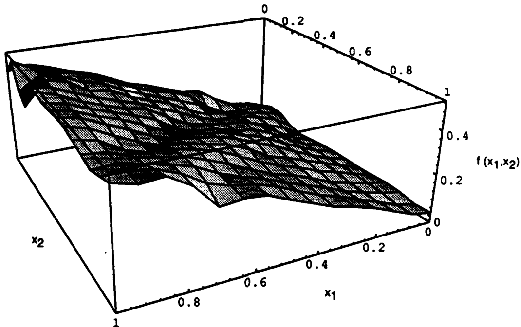
Figure 7.7: Graph of the function f' learned by the recurrent network for one-dimensional segmentation.
