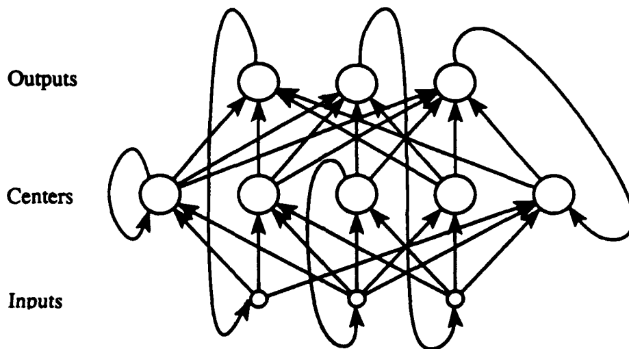
Figure 2.3: Example of a recurrent network
