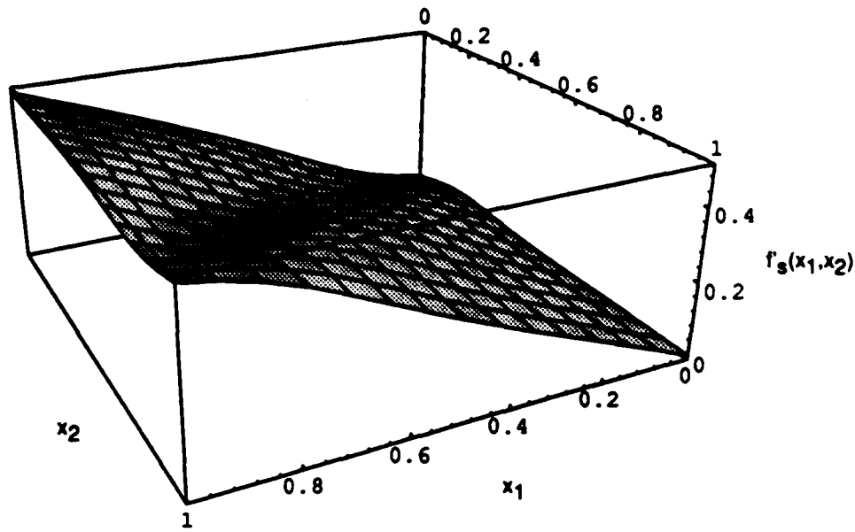
Figure 7.22: Graph of the function f'_s used for the smooth segmentation mapping.
