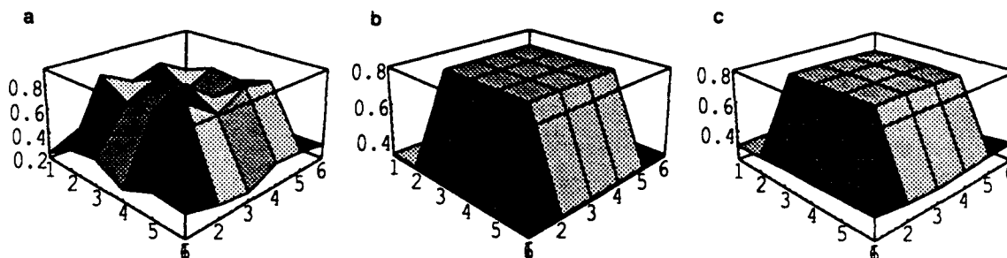
Figure 7.16: a) Input image not used in training the recurrent network. b) Target output image. c) Output of the recurrent network trained to learn two-dimensional segmentation. The network was iterated for ten time steps.
