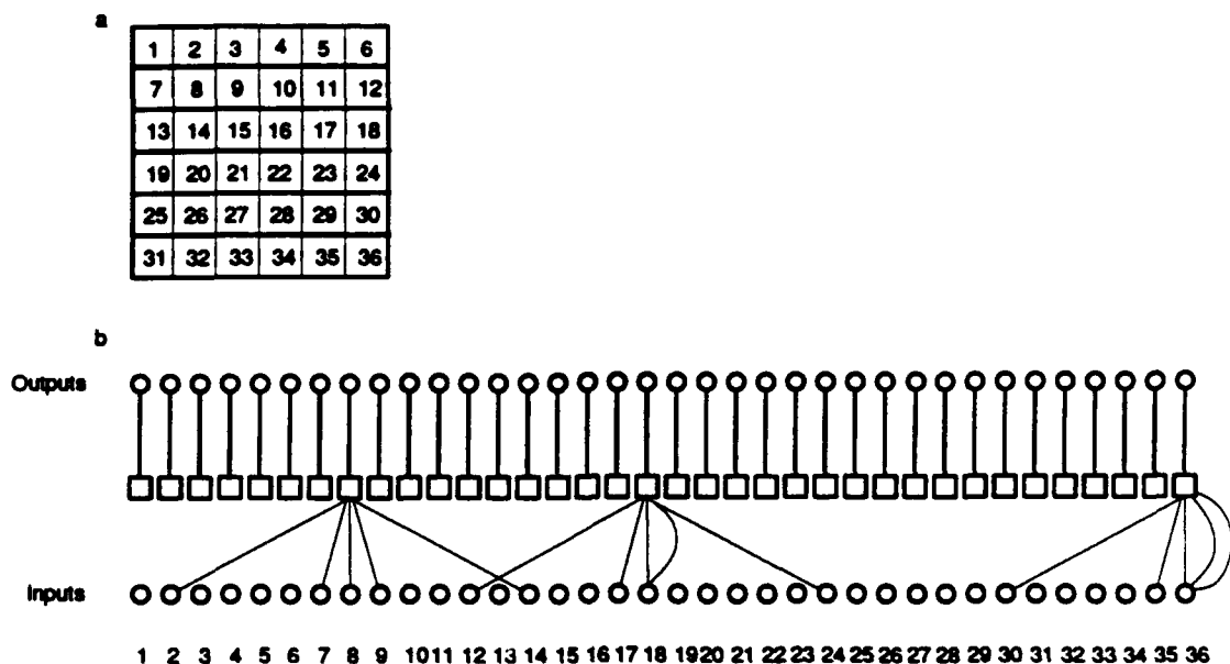
Figure 7.12: a) The pixels of a 6 \times 6 image were numbered as shown so that the images could be given to the recurrent network as one-dimensional vectors. b) This recurrent network was used to learn the two-dimensional segmentation mapping. Each box contains a copy of the function f whose representation is shown in figure 7.11. Only the connections for three of the f boxes are shown so that the figure is less cluttered. The f boxes for boundary pixels such as 18 and 36 that are missing some neighbors compensate by having extra inputs from themselves. Also, the feedback connections from outputs to inputs are not shown.
