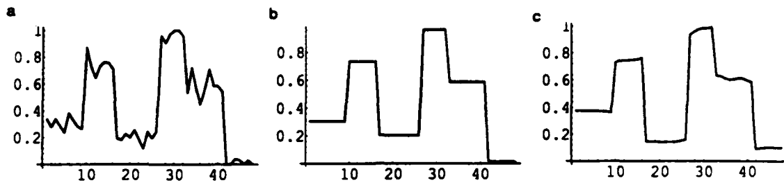
Figure 7.8: a) Input vector obtained by combining three length 16 input vectors which the recurrent network was trained on. b) Target output vector. c) Output of the recurrent network that was trained to learn one-dimensional segmentation. The network was iterated for eight time steps to get this output.
