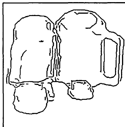
Figure 4.8: Changing edge maps produced by our deterministic MRF-like averaging scheme with a "line process updating" mechanism. Top Left: Original image. Top Right: Initial edge map. Center Left: Edge map after 10 iterations. Center Right: After 20 iterations. Bottom Left: After 50 iterations. Bottom Right: After 100 iterations.
