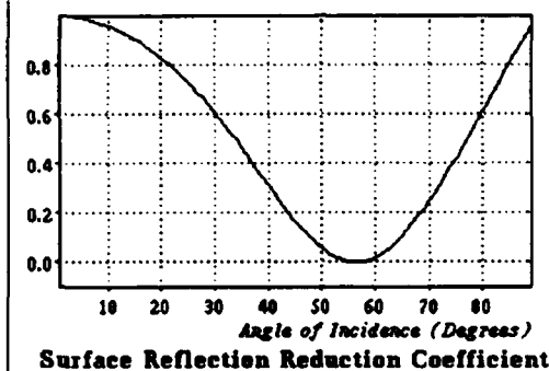
Figure 2.5: Fraction of Remaining Highlight after Polaroid Filtering as a function of Angle of Incidence ( n_t = 1.5 ).
