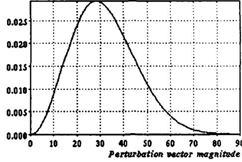
Figure 4.2: Perturbation magnitude (Equation 4.3) for \sigma = 20 . In general, the function peaks at p = \sqrt{2}\sigma .
