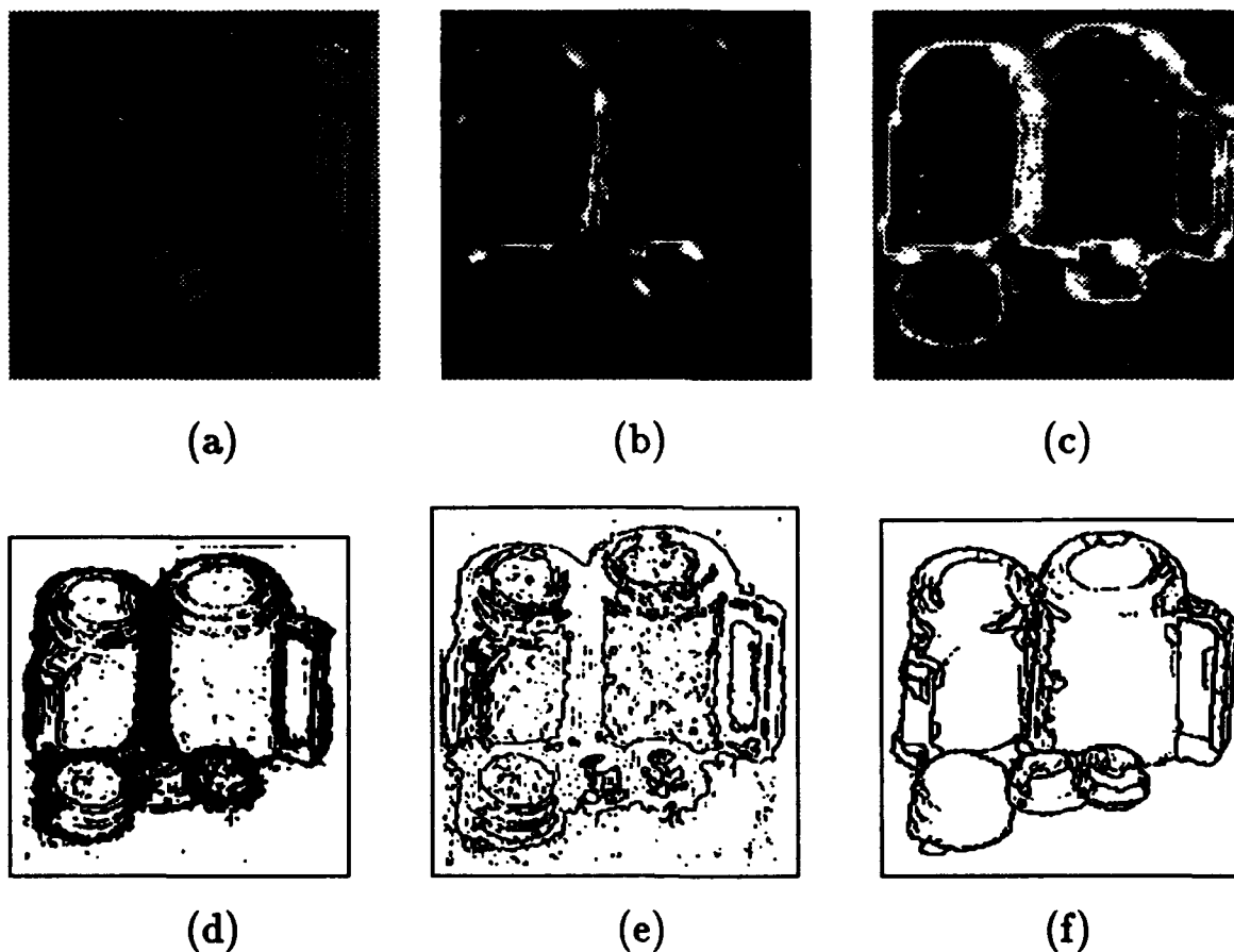
Figure 6.5: Segmentation results obtained from our color region finding algorithm. (a) Image of a plastic scene. (b) Local angular color noise strength. Brighter patches indicate noisier pixels. (c) Relative minimum "detectable patch" widths. Brighter pixels indicate wider patches. (d) Interior pixels. (e) Image "seeds" obtained from linking adjacent "interior pixels". (f) Final regions.
