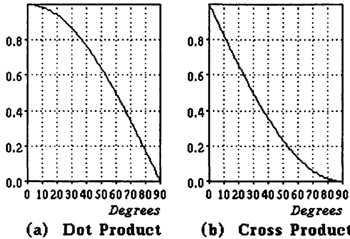
Figure 7.5: Similarity Measure as a Function of Angular Difference for using: (a) Normalized Vector Dot Products, and (b) Normalized Vector Cross Products.
