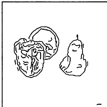
Figure 4.7: Changing edge maps produced by our deterministic MRF-like averaging scheme with a "line process updating" mechanism. Top Left: Original image. Top Right: Initial edge map. Center Left: Edge map after 10 iterations. Center Right: After 20 iterations. Bottom Left: After 50 iterations. Bottom Right: After 100 iterations.
