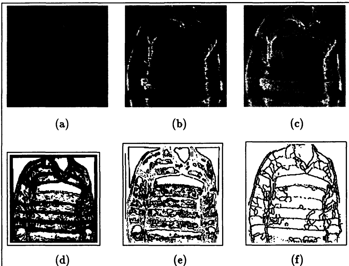
Figure 6.4: Segmentation results obtained from our color region finding algorithm. (a) Image of a color striped sweater. (b) Local angular color noise strength. Brighter patches indicate noisier pixels. (c) Relative minimum "detectable patch" widths. Brighter pixels indicate wider patches. (d) Interior pixels. (e) Image "seeds" obtained from linking adjacent "interior pixels". (f) Final regions.
