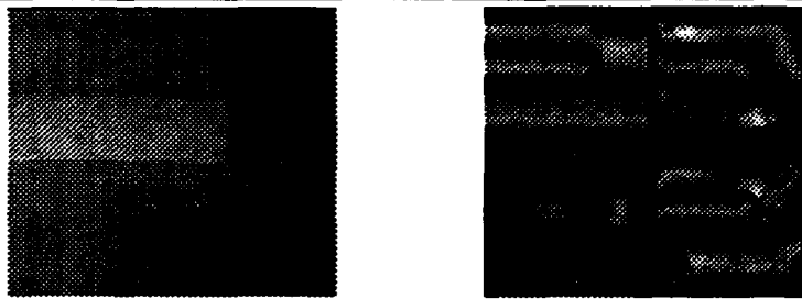
Figure 7.13: Left: Image of 3 rectangular regions. Right: "Insideness" or Inertia maps for the rectangular regions. From the top-left in a clockwise direction, the reference directions are: North-South, East-West, Northeast-Southwest and Northwest-Southeast. Brighter points have higher inertia values.
