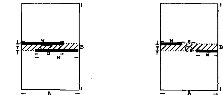
(c) overlapped and non-overlapped antipodal finline
