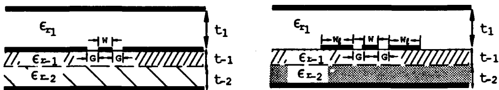
(d) conductor backed coplanar waveguide with infinite/finite lateral ground planes
