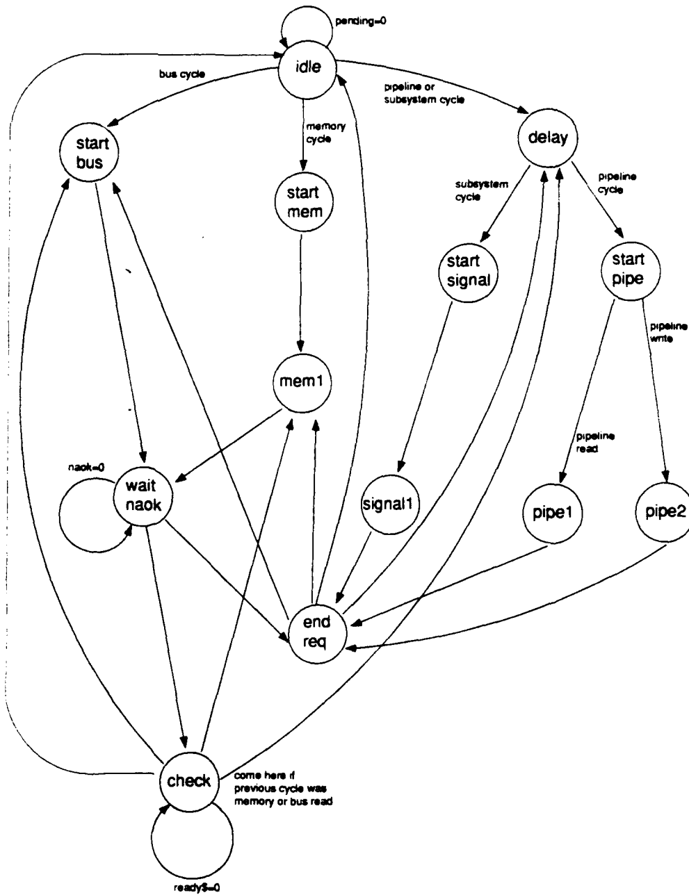
Figure 16. Slave request control state machine
