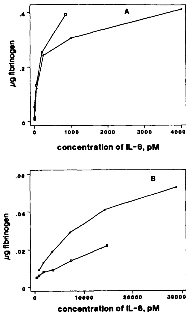
Fig. 1. Dose-response curves of human IL-6 variants in the hepatocyte stimulation assay using human hepatoma cell line. (A) (●) IL-6, native IL-6; (□) IL-6S4-23, deletion mutant of IL-6. (B) (●) IL-6S, serine-substituted IL-6; (□) IL-6S4-23, deletion mutant of IL-6S.
