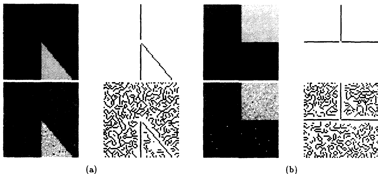
Figure 14: For the junction in figures (a), vanishing gradients increase \frac{\partial^2}{\partial n^2} 's sensitivity to noise, as seen in the Canny edges to the immediate right – notice the gap introduced at the junction when the noise is added. Vanishing gradients do not affect the junction on the right (b), so adding noise does not add any new gaps in the edge map.
