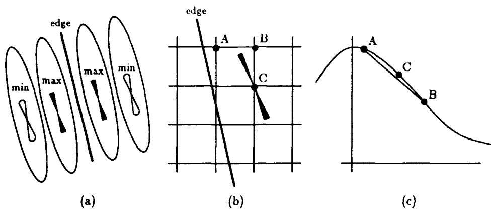
Figure 18: (a) The layers of min and max bow ties surrounding an edge; (b) The max bow tie at C depends on the linear interpolation between A and B; (c) The interpolated points between A and B fall below the Gaussian in its concave down section.
