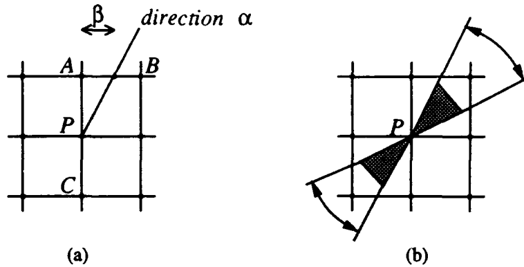
Figure 16: (a) We use linear interpolation between A and B to calculate the value of the gradient magnitude in direction \alpha : the interpolated value = \beta B + (1 - \beta)A . For the max bow tie in (b), |\nabla f| at P is bigger than the indicated interpolated values.
