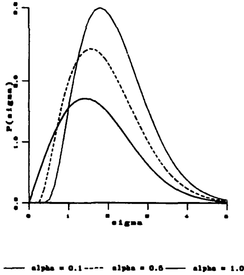
Figure 4: The distribution of variance \tilde{P}(\sigma) associated to the multiquadric effective potential.
