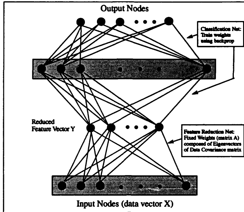
Figure 2.5. Network Architecture for Karhunen-Loève Feature Extractor. (37)
