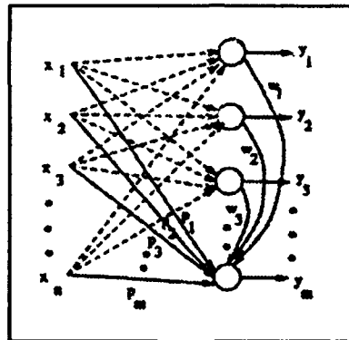
Figure 2.2. APEX network: solid lines denote weights p_i, w_j and are trained at the m^{\text{th}} stage. (Note that w_j asymptotically approach zero as the network converges) (17).
