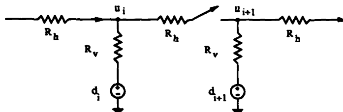
Figure 12: Resistive fuse network for solving discrete variational problem of equation (11). Horizontal elements behave as linear resistors for small voltages across their terminals, but are open-circuits if the voltage difference is too large.
