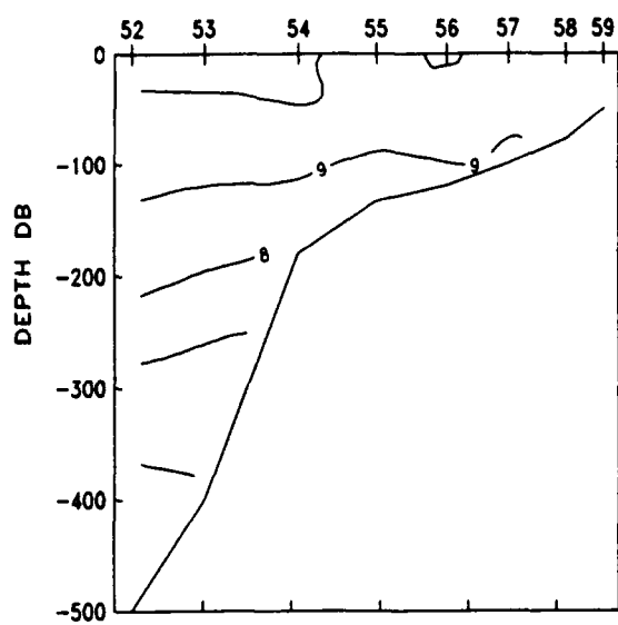
B TEMPERATURE
