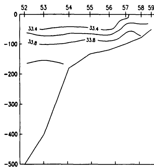
B SALINITY
